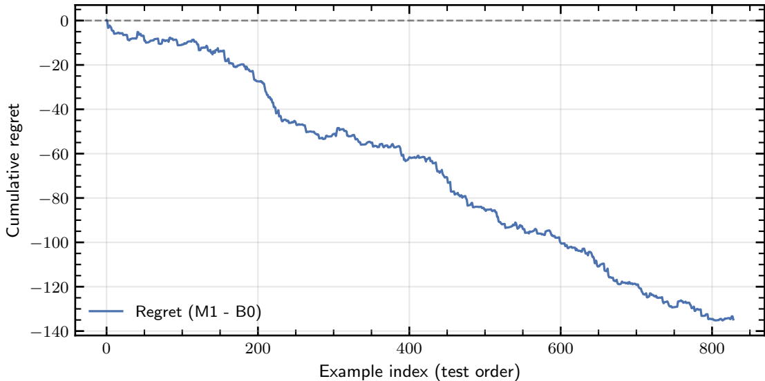
Cumulative Regret vs Baseline
