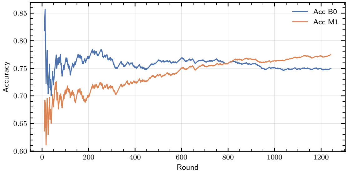
Training Accuracy (Cumulative)
