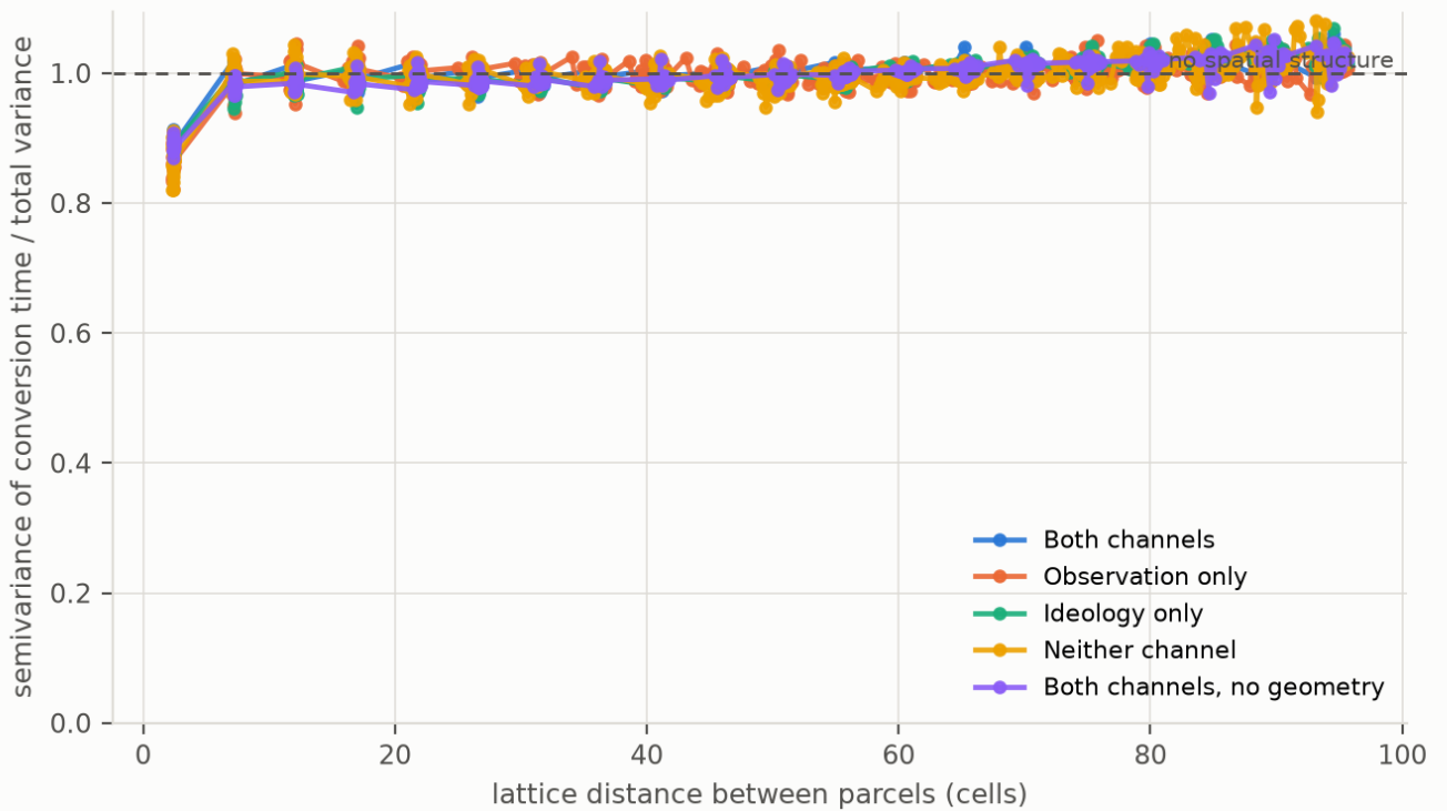
Figure 6: The semivariogram of first-conversion time: half the mean squared difference in conversion time between pairs of parcels, against the lattice distance separating them, normalised by the total variance. No origin is assumed. A curve rising from a low value at short distance is a spreading front, and the distance at which it flattens is the spatial scale of the process. A flat line at unity throughout is simultaneity: parcels one cell apart convert as differently as parcels a country apart.
