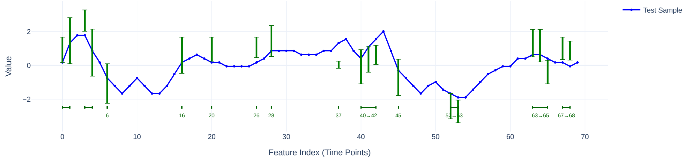
Maximal REASON (cost=14.3286, 13 intervals)
