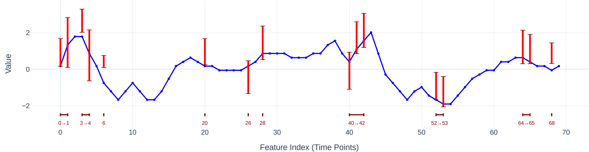
Maximal ANTI-REASON (cost=17.5626, 10 intervals)
