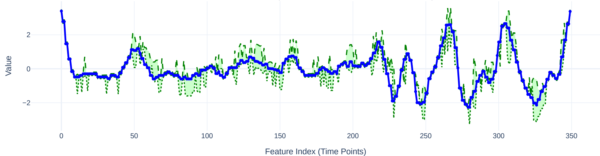
Maximal REASON (cost=148.1676, 151/350 constrained)
