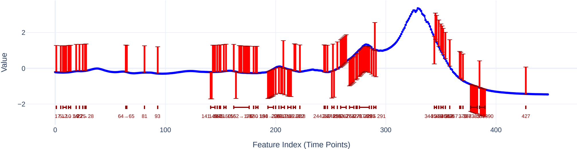
Maximal ANTI-REASON (cost=84.0598, 45 intervals)
