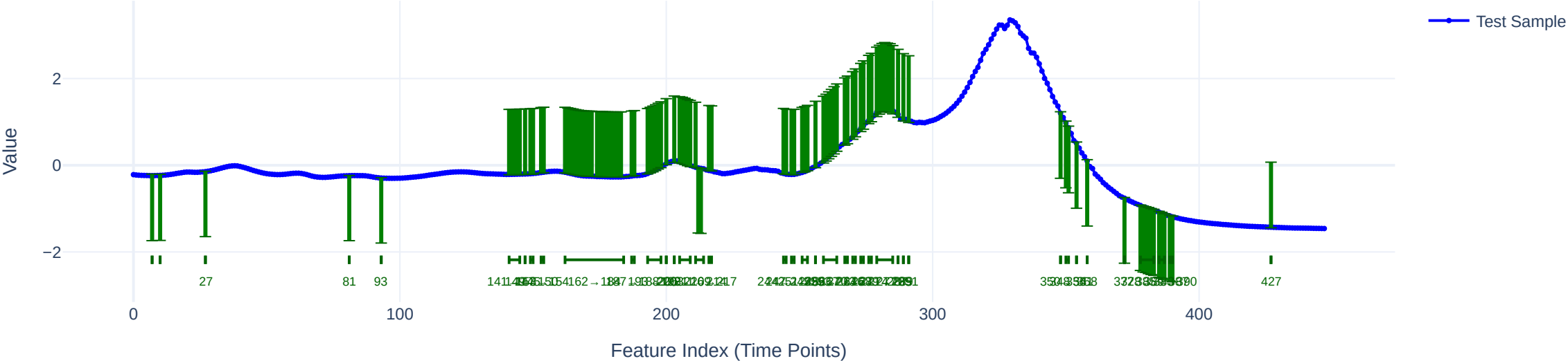
Maximal REASON (cost=131.0879, 39 intervals)
