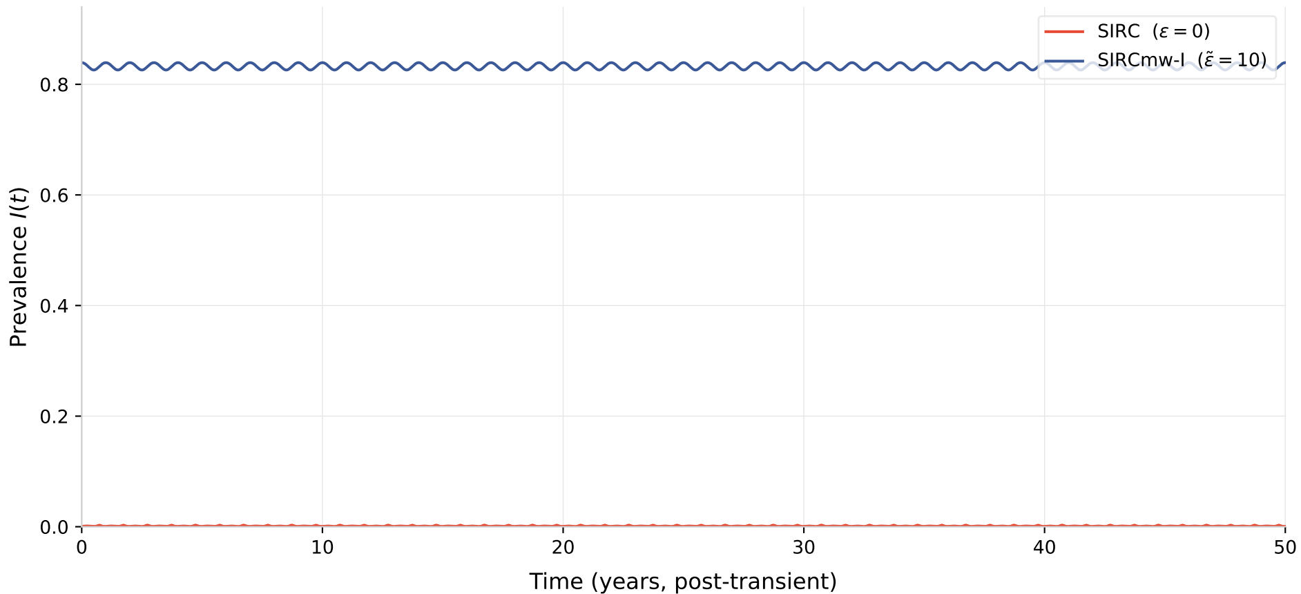
Seasonally-Forced SIRC vs SIRCmw-I ( \eta = 0.07 , \beta_0 = 1200.0 , \varepsilon_1 = \varepsilon_2 = \varepsilon )
