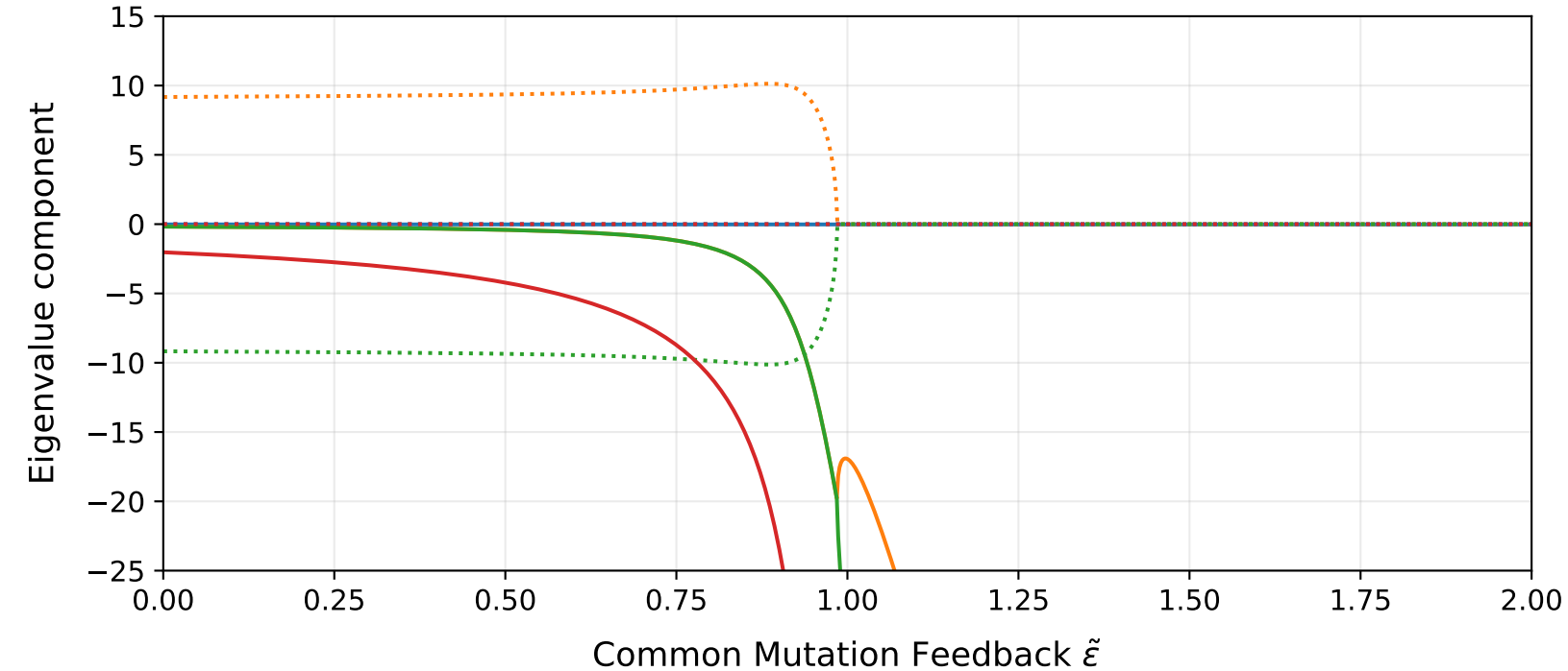
Zoomed Spectrum ( \tilde{\epsilon} \in [0.0, 2.0] , \lambda \in [-25, 15] )
