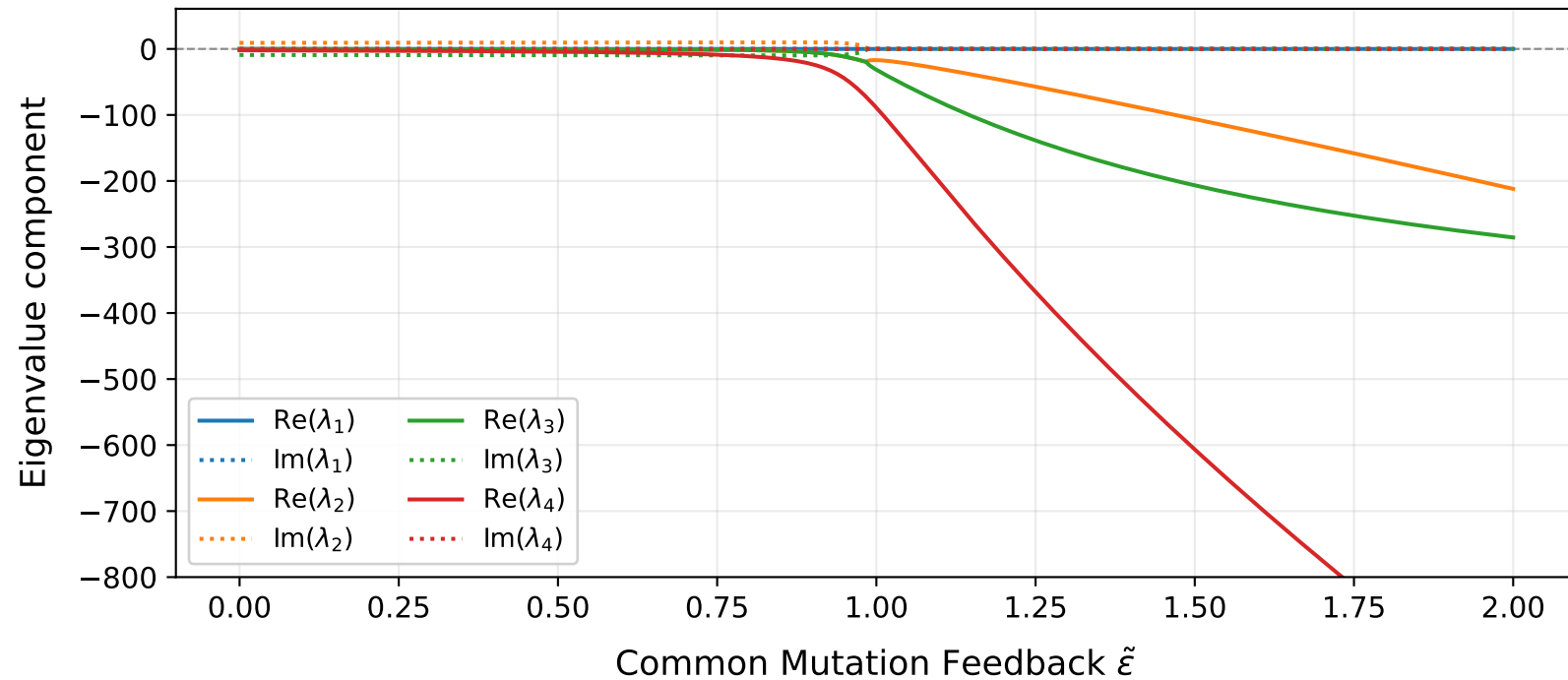
Full Jacobian Spectrum ( \beta_0 = 600 )
