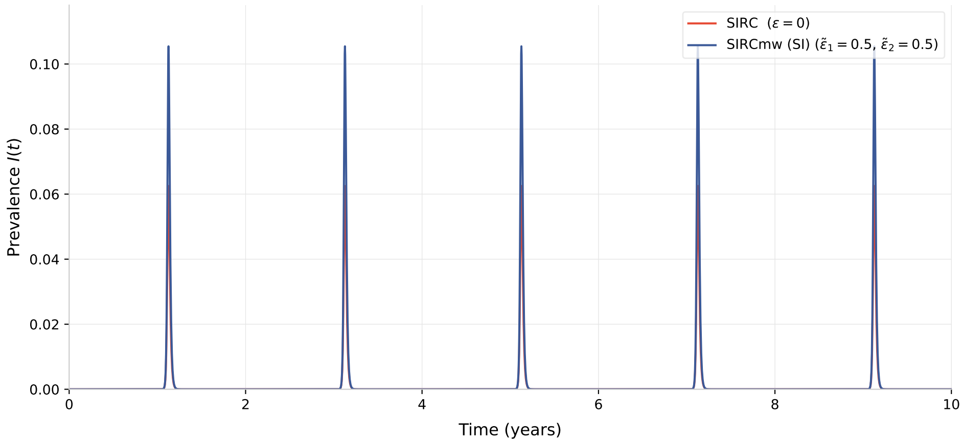
Seasonally-Forced SIRC vs SIRCmw (SI version) ( \eta = 0.28 , \beta_0 = 600.0 )
