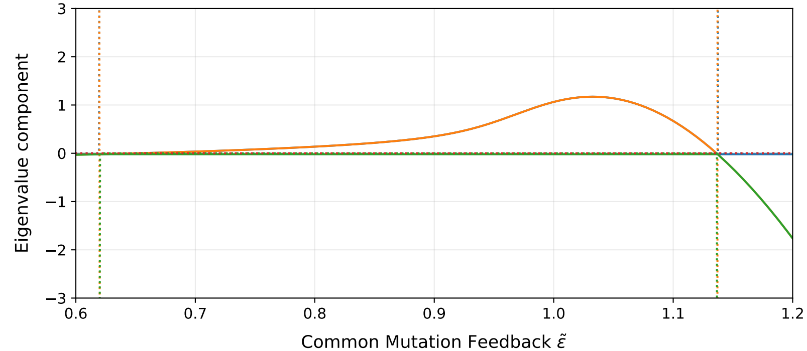
Zoomed Spectrum ( \tilde{\epsilon} \in [0.6, 1.2] , \lambda \in [-3, 3] )
