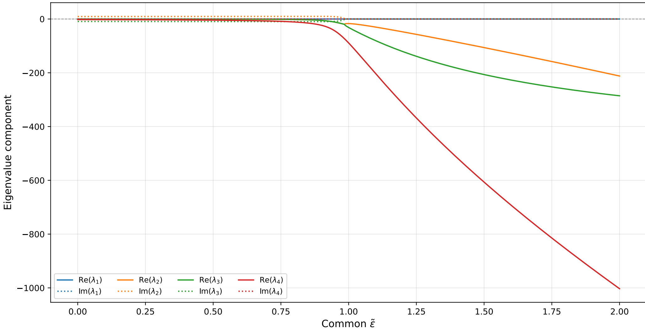
SIRCmw eigenvalues at endemic equilibrium ( \beta_0 = 600 )
