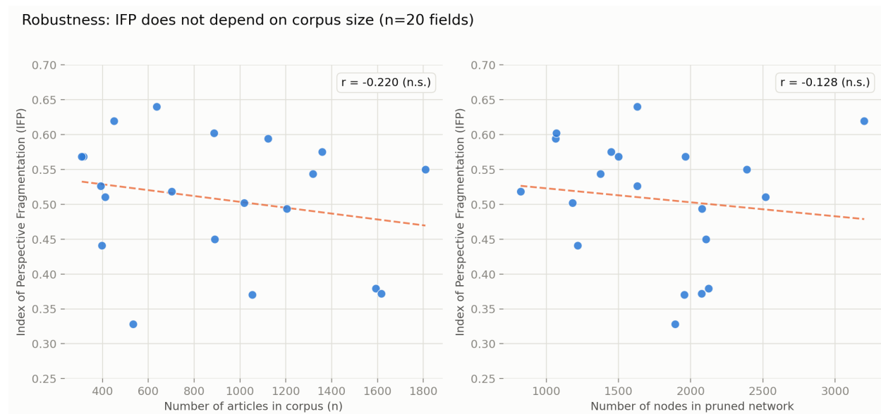
Figure 7: Robustness check: IFP plotted against the number of source articles (left) and the number of nodes in the pruned network (right), across all 20 fields. Dashed lines show ordinary least-squares fits; neither correlation is statistically significant at \alpha = 0.05 .
