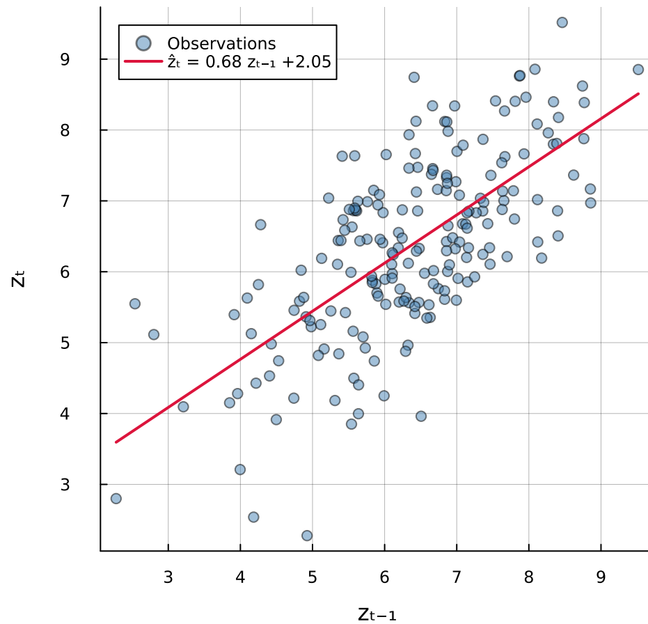
Least-squares regression
