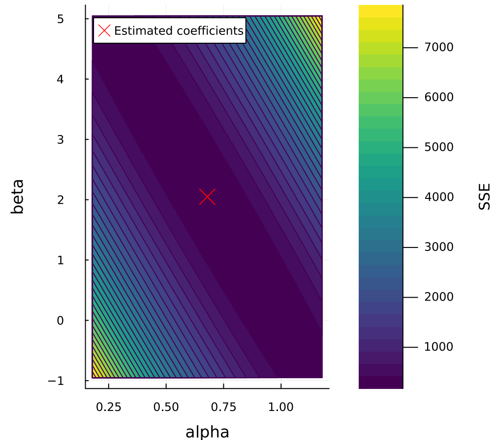
Sum of squared errors
