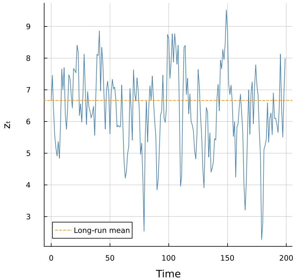
AR(1) time series
