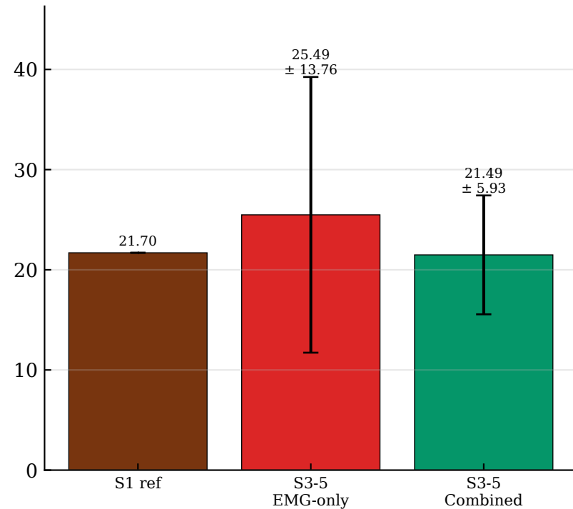
Noise floor (uV)
