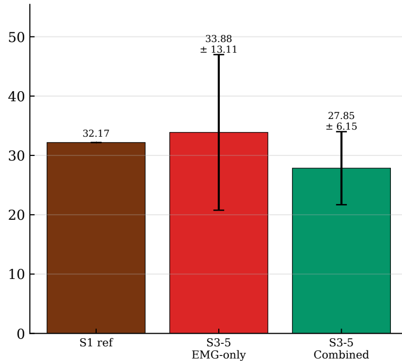
Contraction RMS (uV)
