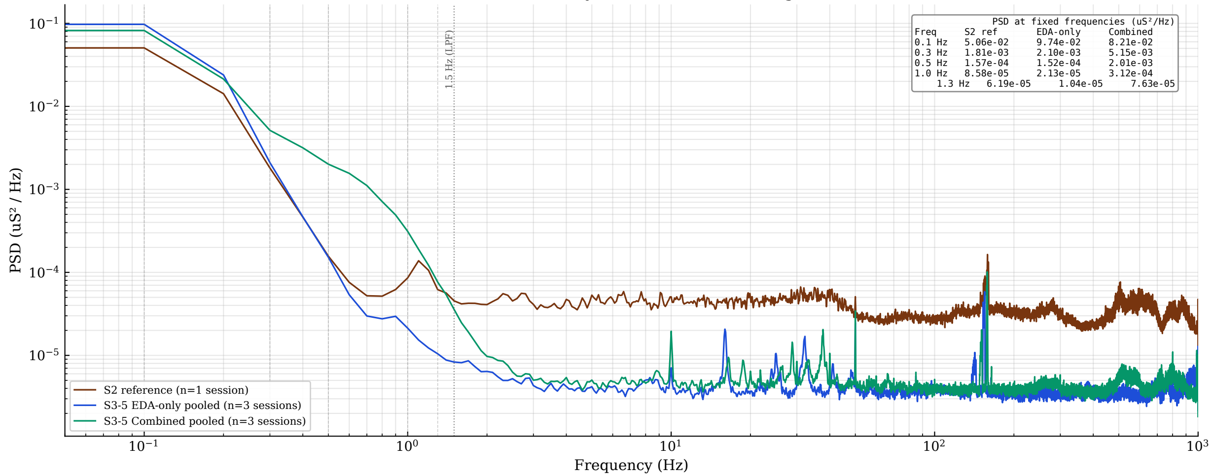
Q5: EDA PSD by condition (full recording)
