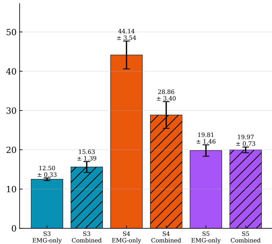
Noise floor (uV)
