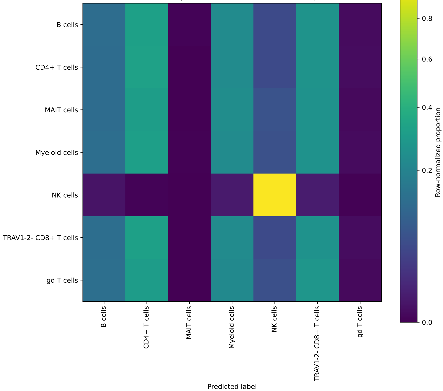
Blood Atlas: pooled donor-held-out confusion (PCA)
