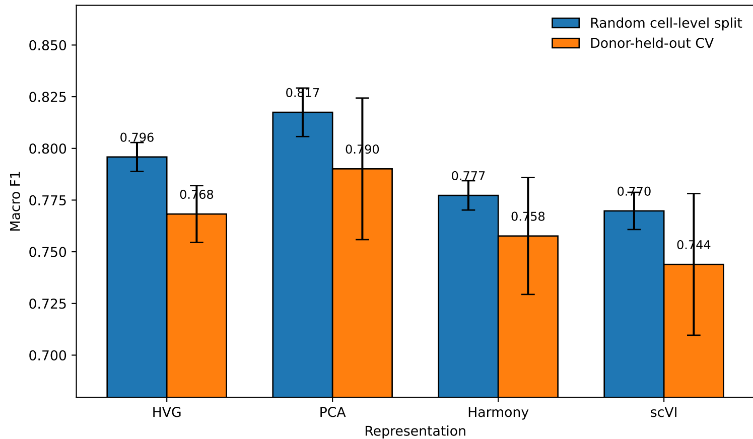
PBMC: random vs donor-held-out evaluation
