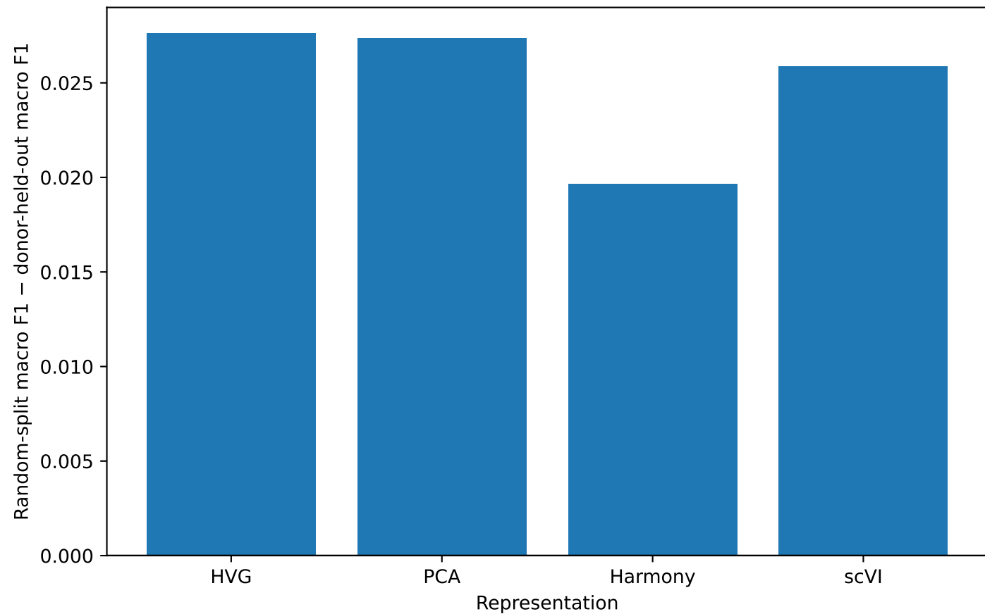
PBMC: evaluation inflation
