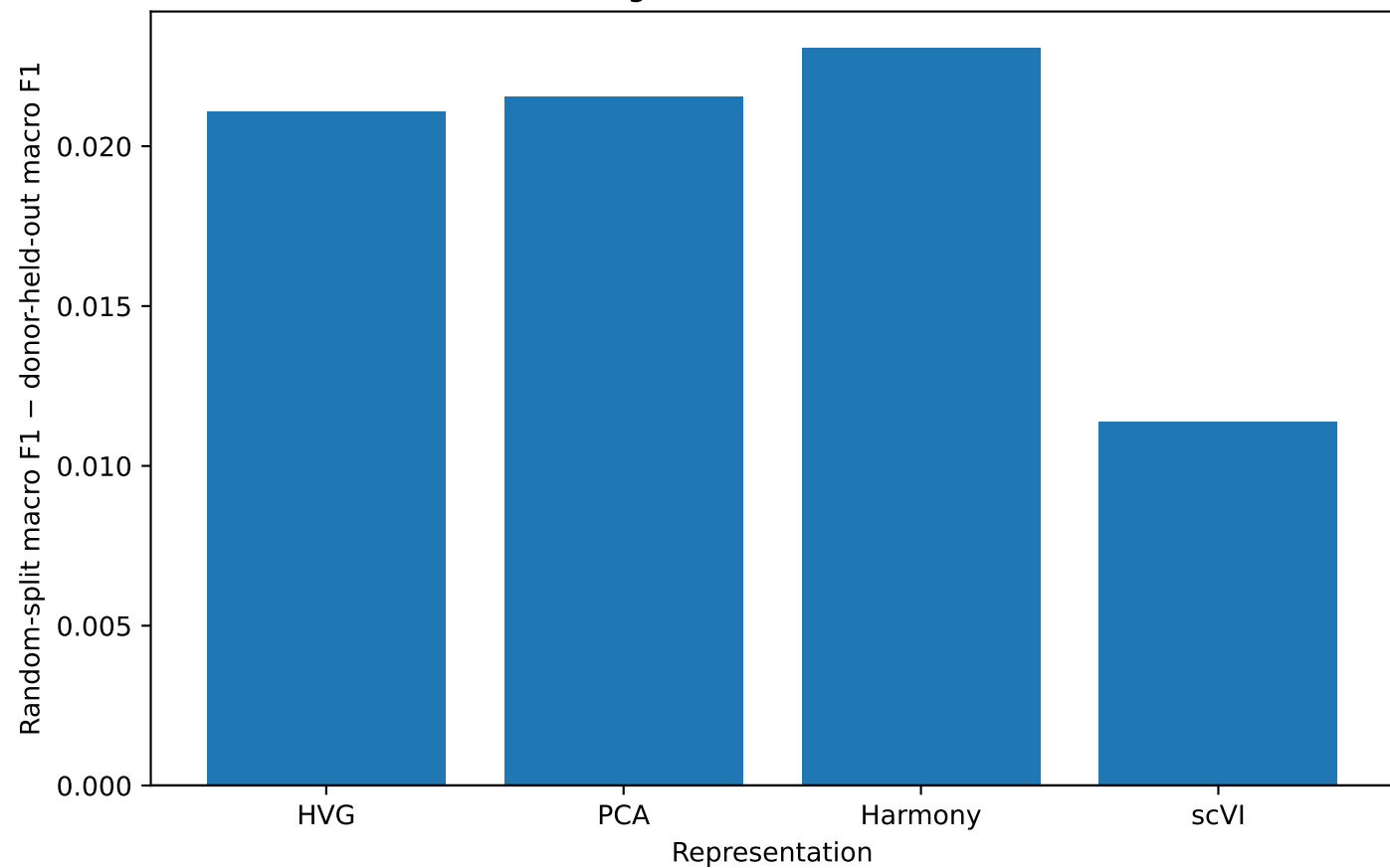
Lung: evaluation inflation
