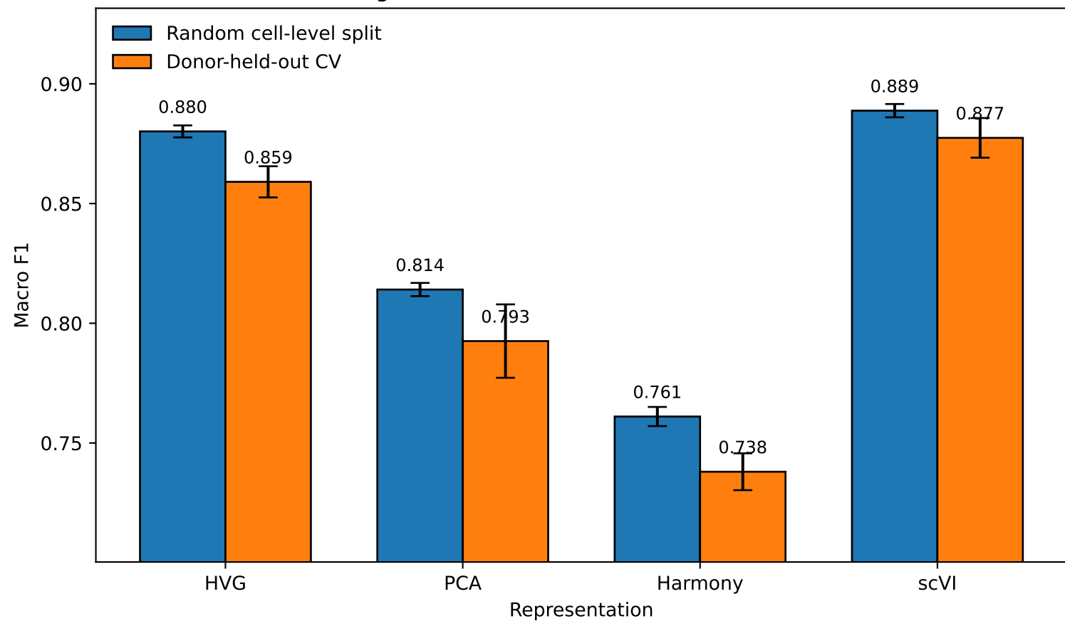
Lung: random vs donor-held-out evaluation
