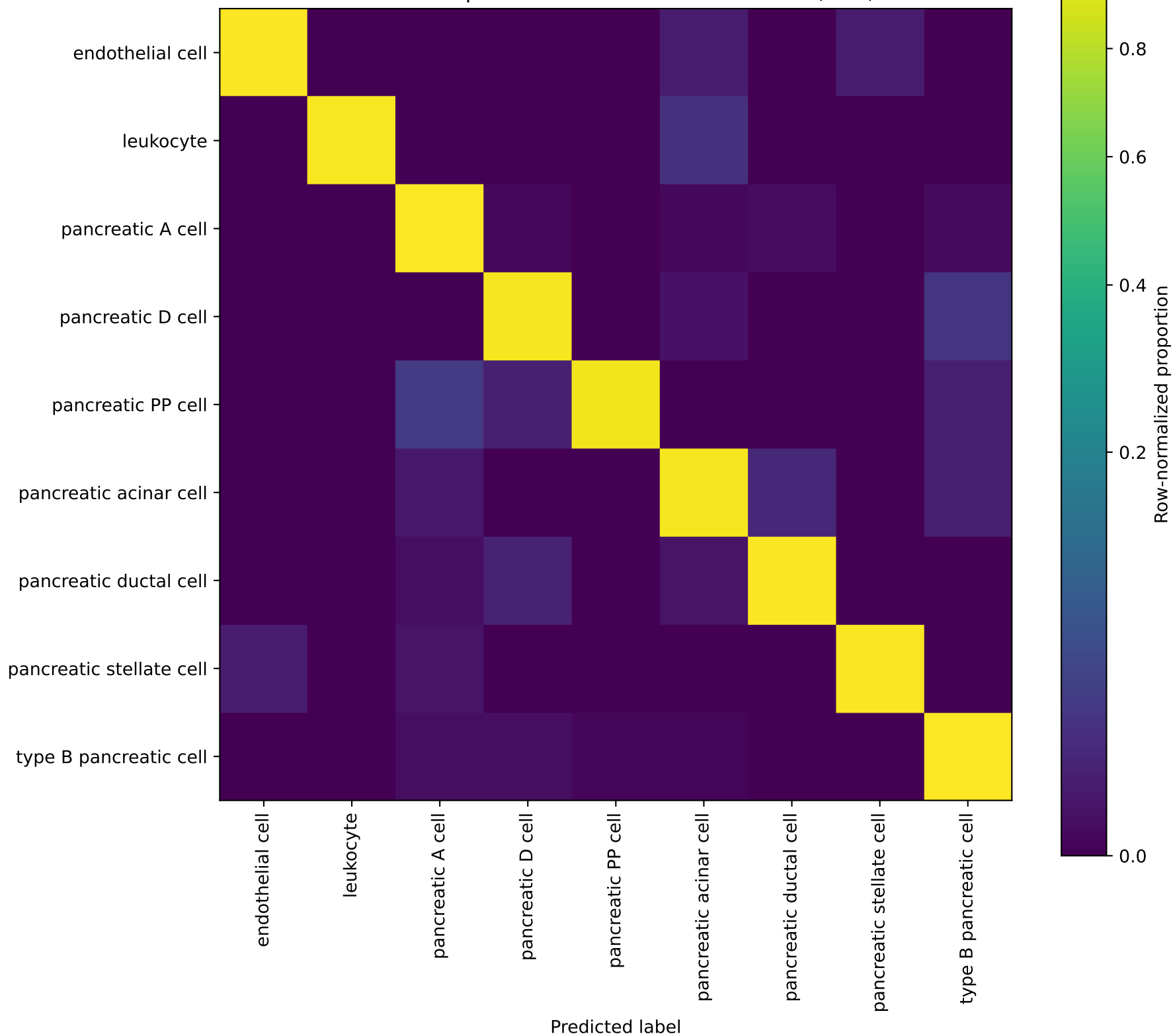
Pancreas: pooled donor-held-out confusion (scVI)
