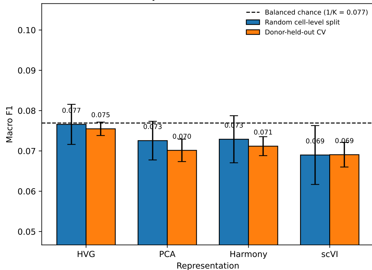
A. Synthetic-label floor control
