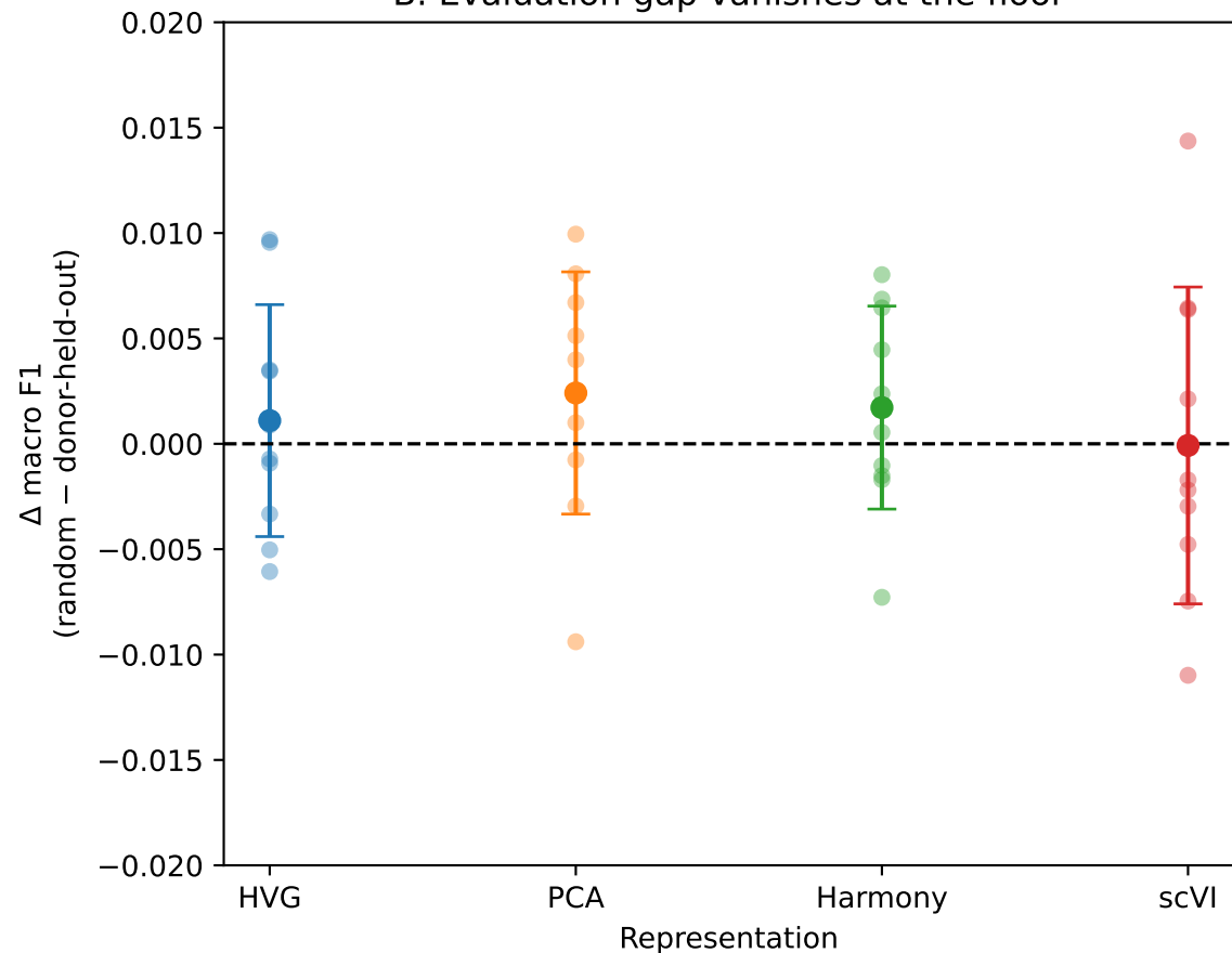
B. Evaluation gap vanishes at the floor
