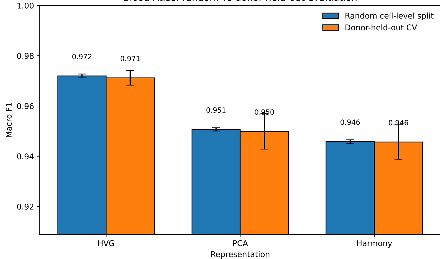
Blood Atlas: random vs donor-held-out evaluation
