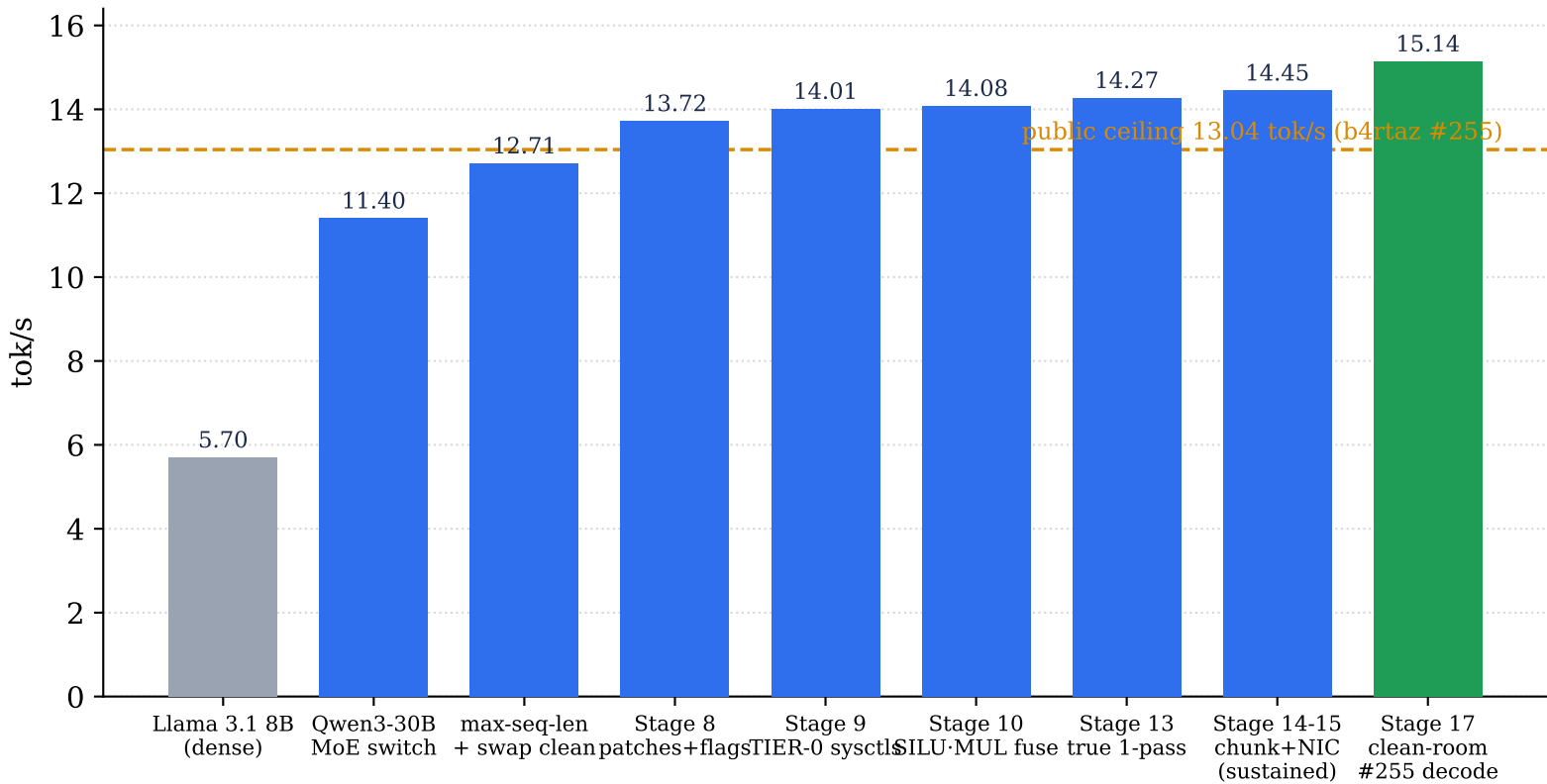
Optimisation trajectory and final clean-room result Qwen3-30B-A3B on 4× Raspberry Pi 5 (last bar: decode rate, telemetry off, +16.1% vs ceiling)
