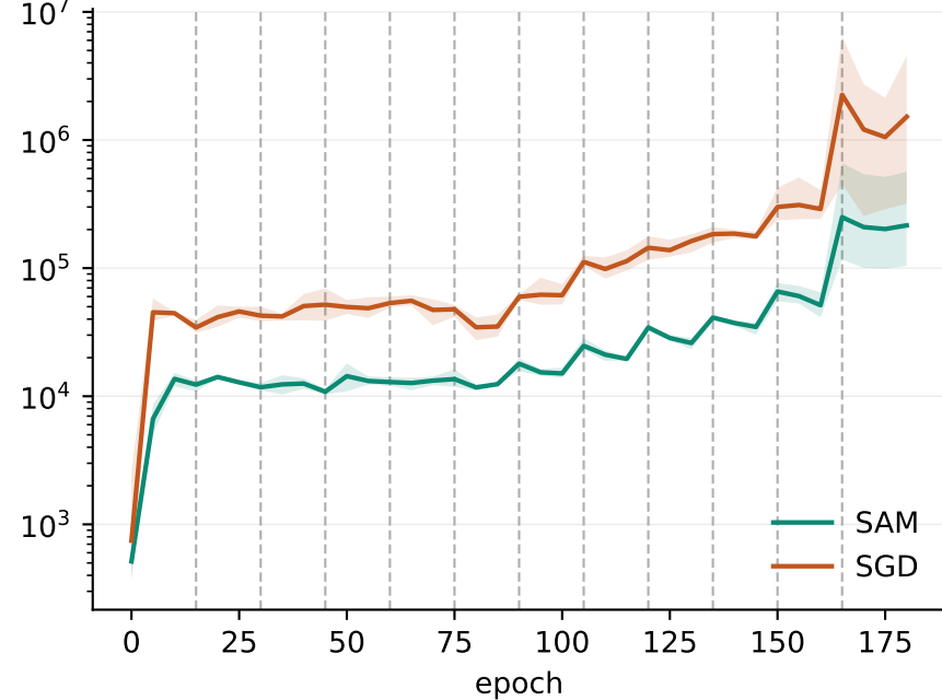
ResNet-18, s = 0.9995
