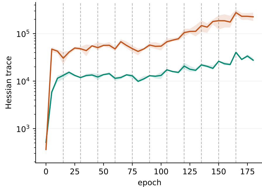
ResNet-18, s = 0.995
