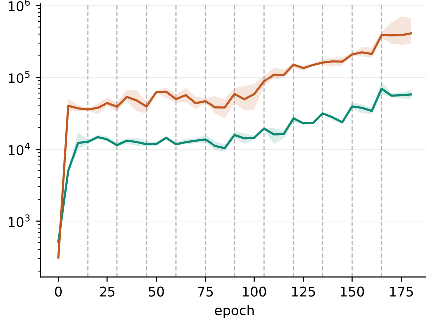
ResNet-18, s = 0.999
