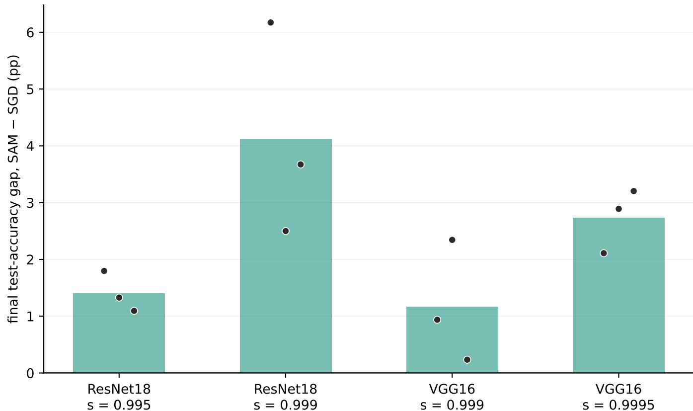
SAM's final-accuracy edge grows with sparsity (bars = mean across 3 seeds; dots = individual seeds)
