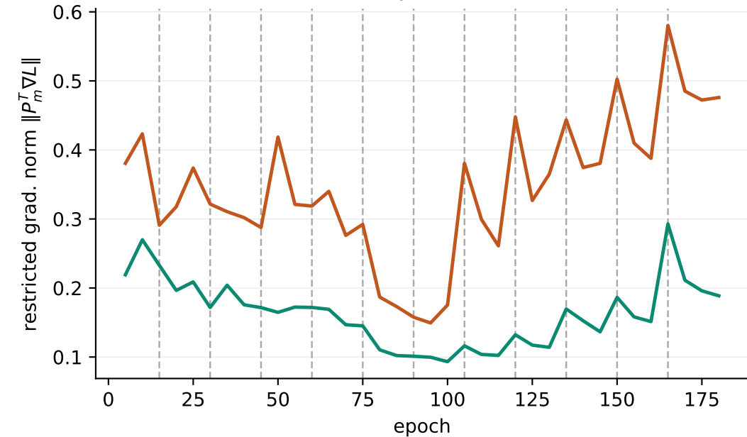
VGG16, s = 0.999
