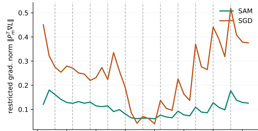
ResNet18, s = 0.995
