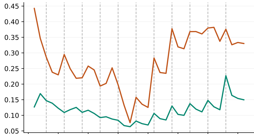
ResNet18, s = 0.999
