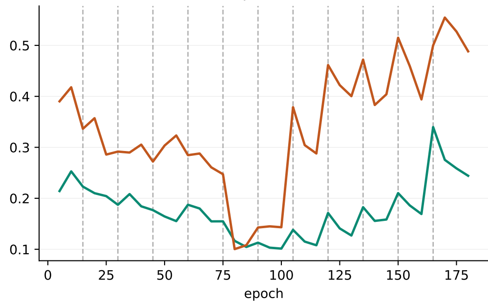
VGG16, s = 0.9995
