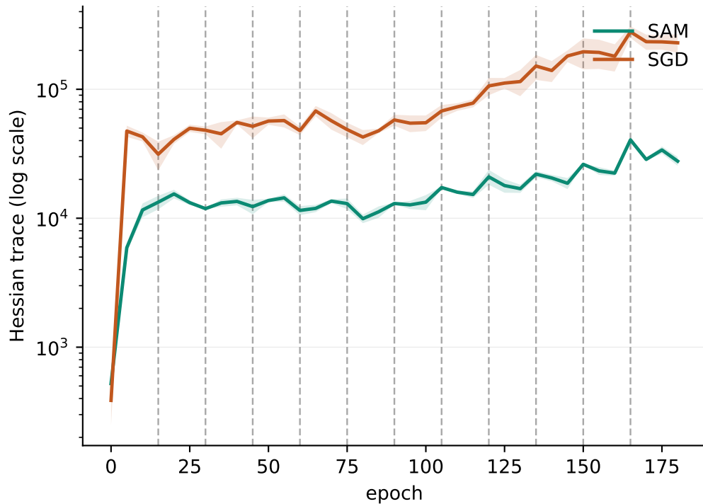
ResNet18, s = 0.995
