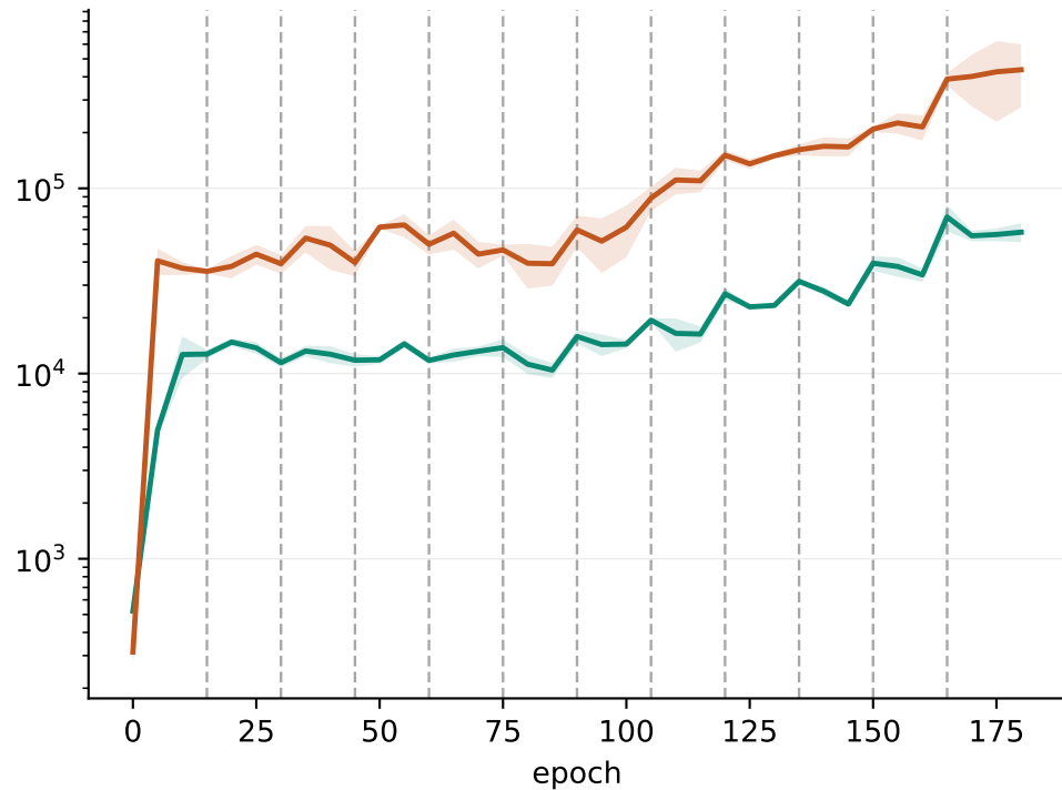
ResNet18, s = 0.999
