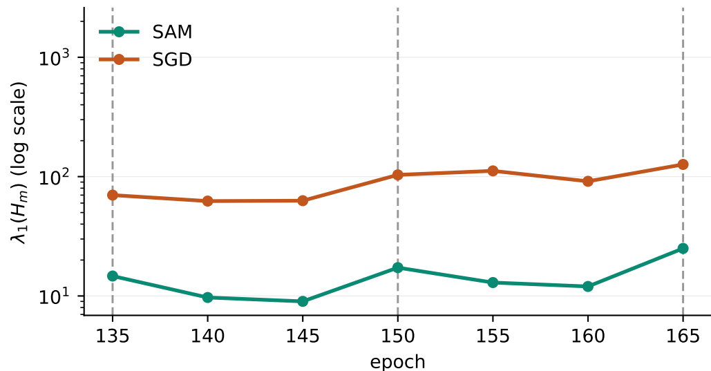
ResNet18, s = 0.995
