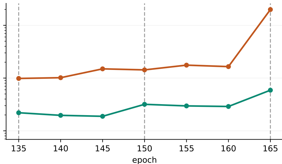
ResNet18, s = 0.999
