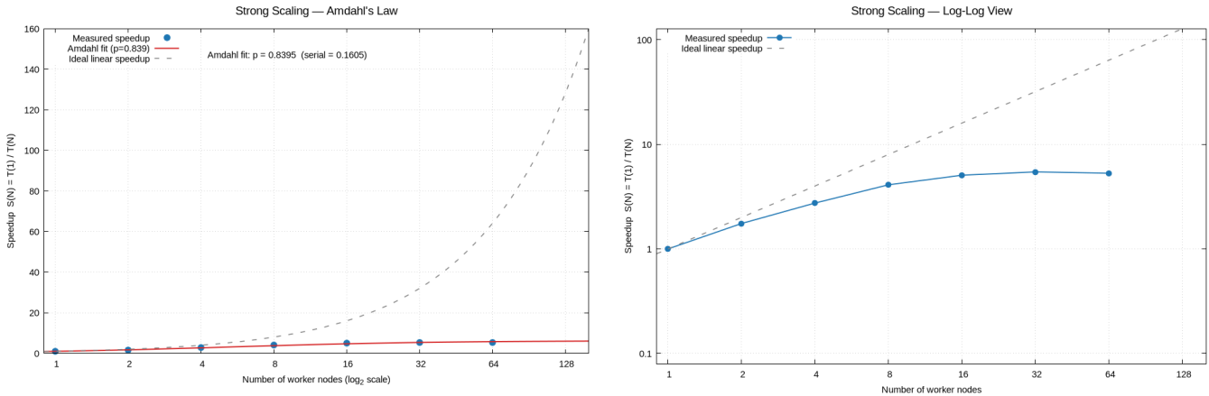
Figure 3: Measured speedup for the 8-chunk CC dataset under the disk-backed architecture. The left figure is the main Amdahl view with linear speedup on the y -axis; the right figure shows the same data on a log-log scale to emphasize the high-node-count collapse.
