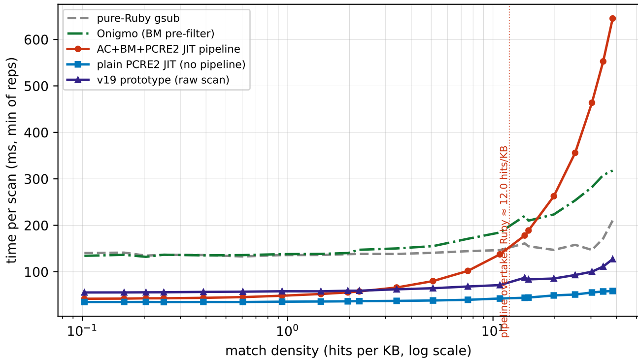
Pre-filter pipeline vs. no pipeline (shippable-class engines)
