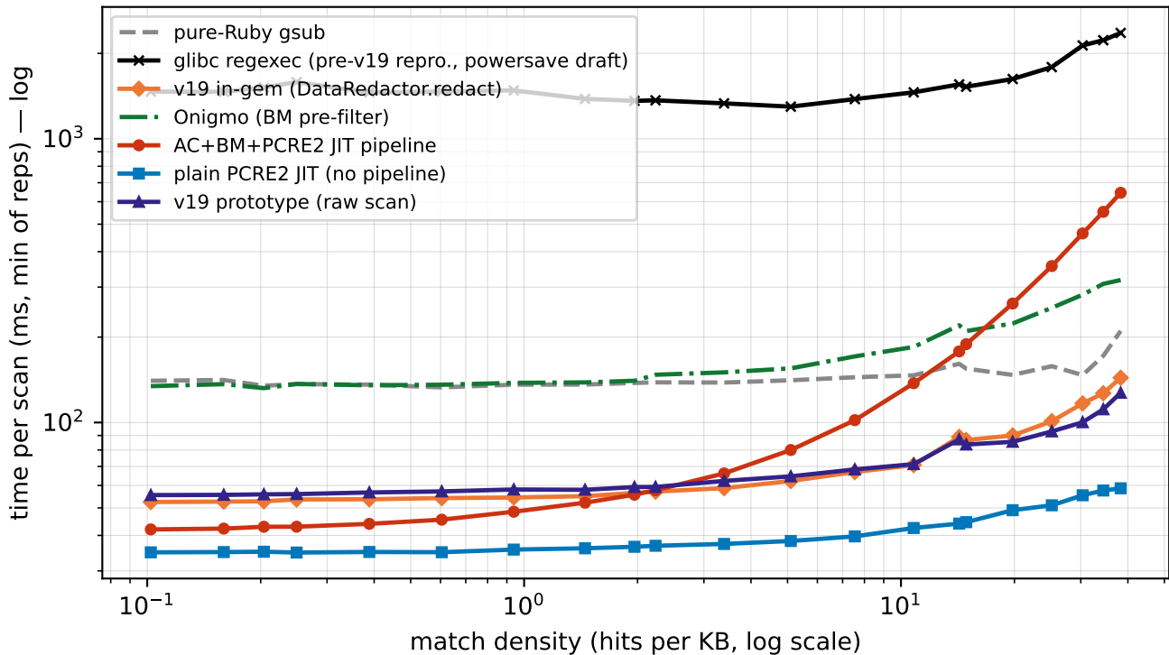
All engines across match density (log time)
