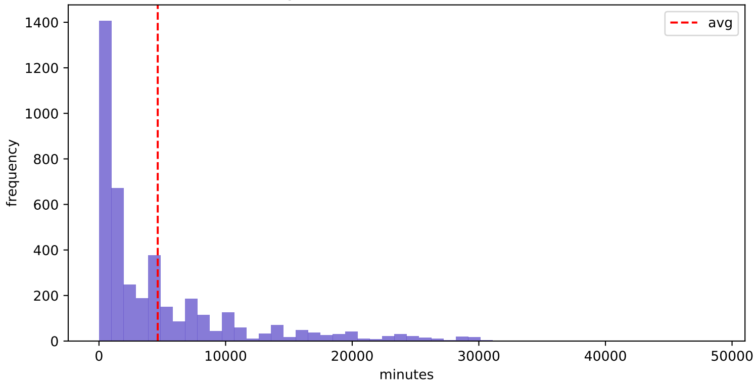
BPIC2017_After - O_Accepted (Avg 4639.69 min, Std 6269.47 min)
