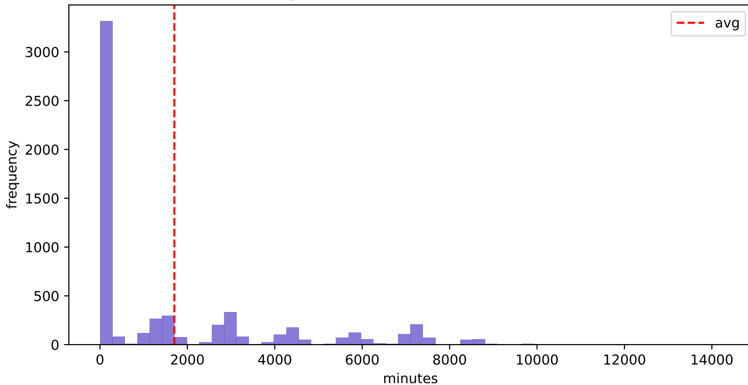
BPIC2017_Before - W_Validate application (Avg 1703.12 min, Std 2478.97 min)
