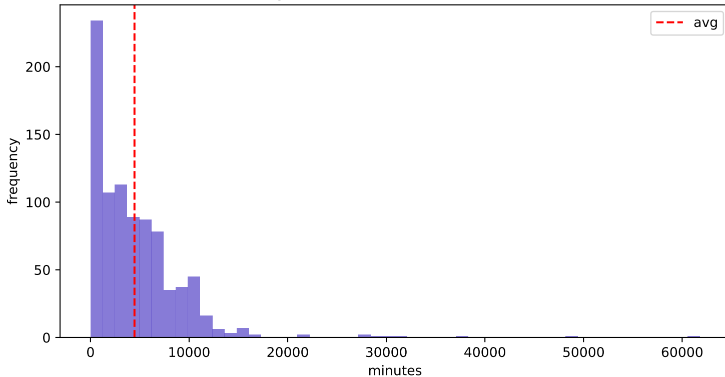
BPIC2017_After - A_Denied (Avg 4459.68 min, Std 4953.46 min)
