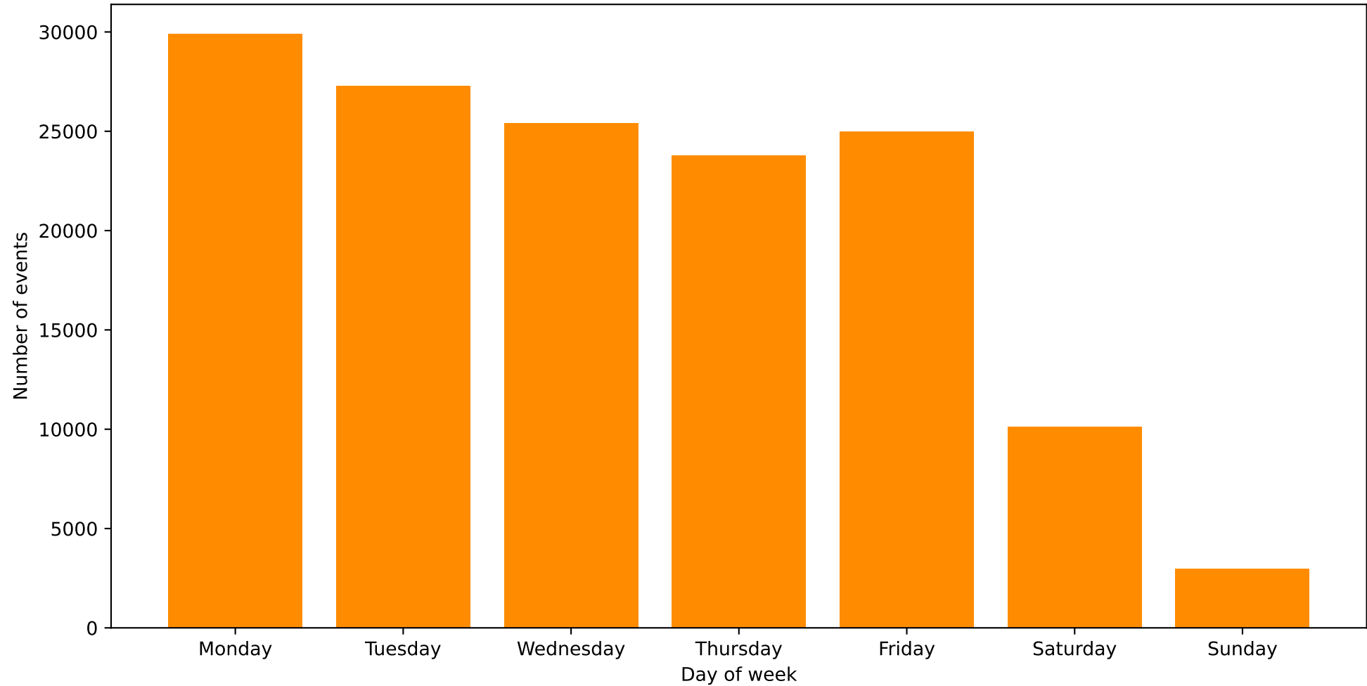
BPIC2017_Before - Role 6 (O_Cancelled) - Working days
