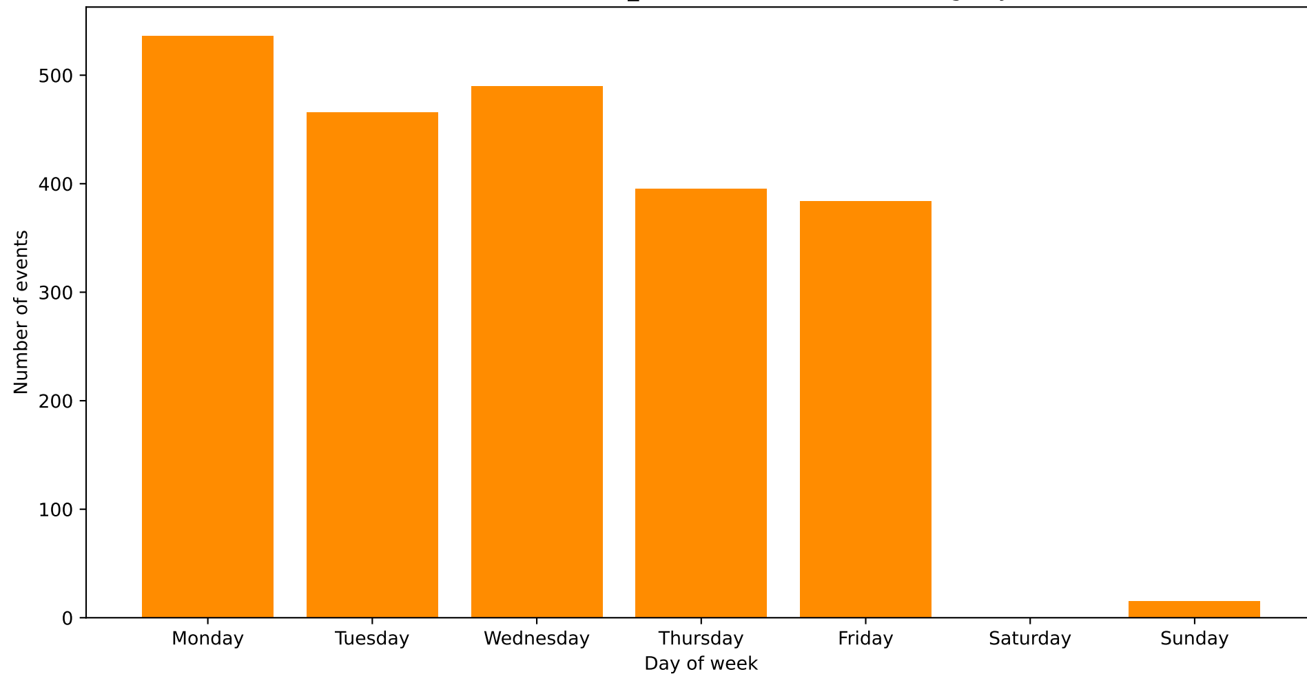
BPIC2012 - Role 11 (W_Beoordelen fraude) - Working days
