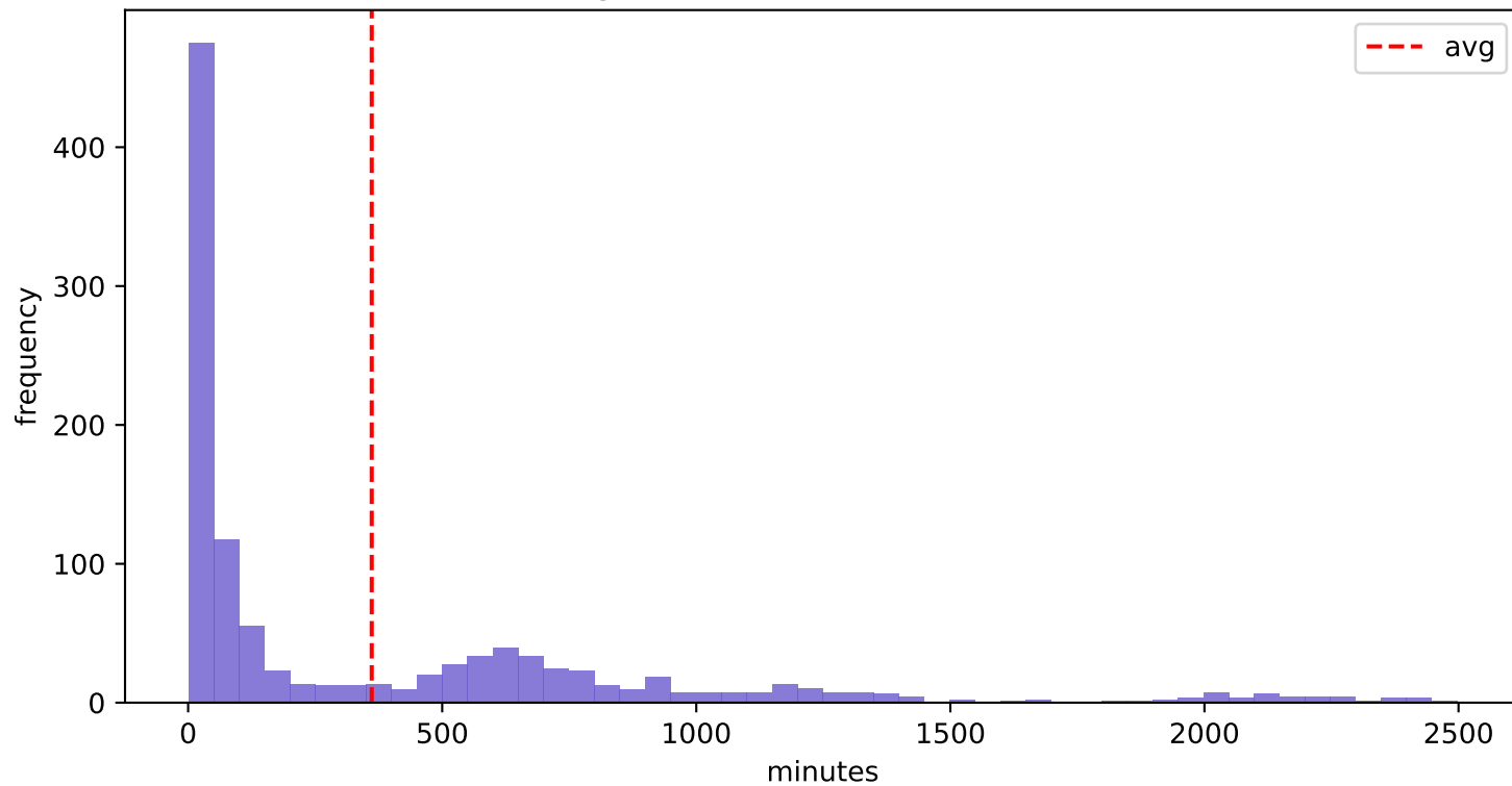
BPIC2017_Before - W_Handle leads (Avg 361.33 min, Std 520.87 min)
