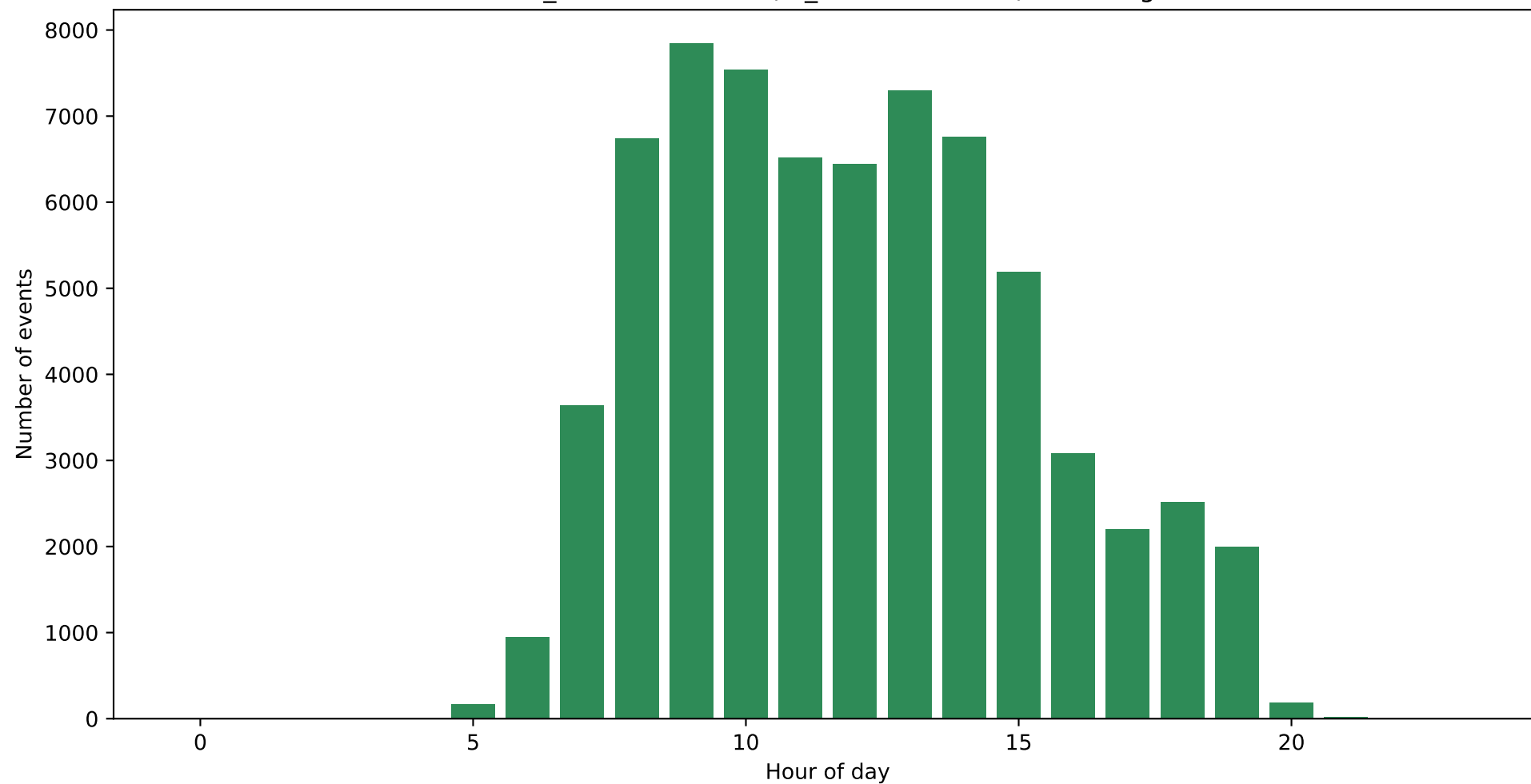
BPIC2017_Before - Role 11 (W_Call after offers) - Working hours
