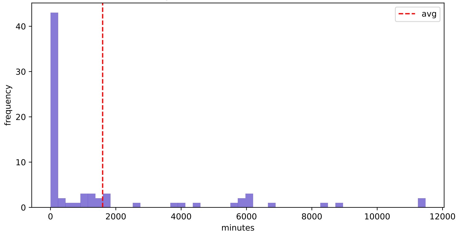
BPIC2017_Before - W_Assess potential fraud (Avg 1597.10 min, Std 2804.77 min)
