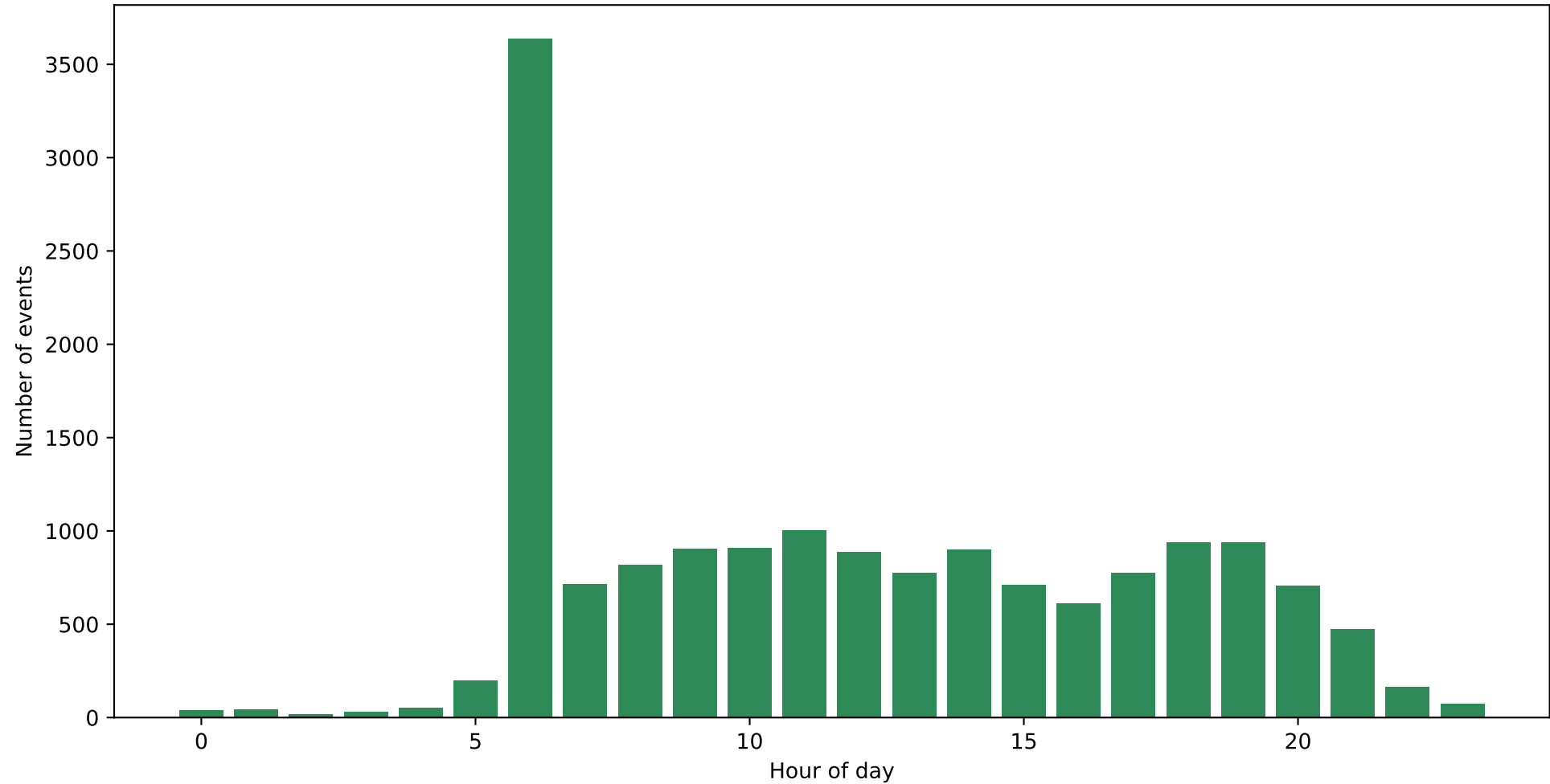
BPIC2017_After - Role 14 (A_Submitted) - Working hours
