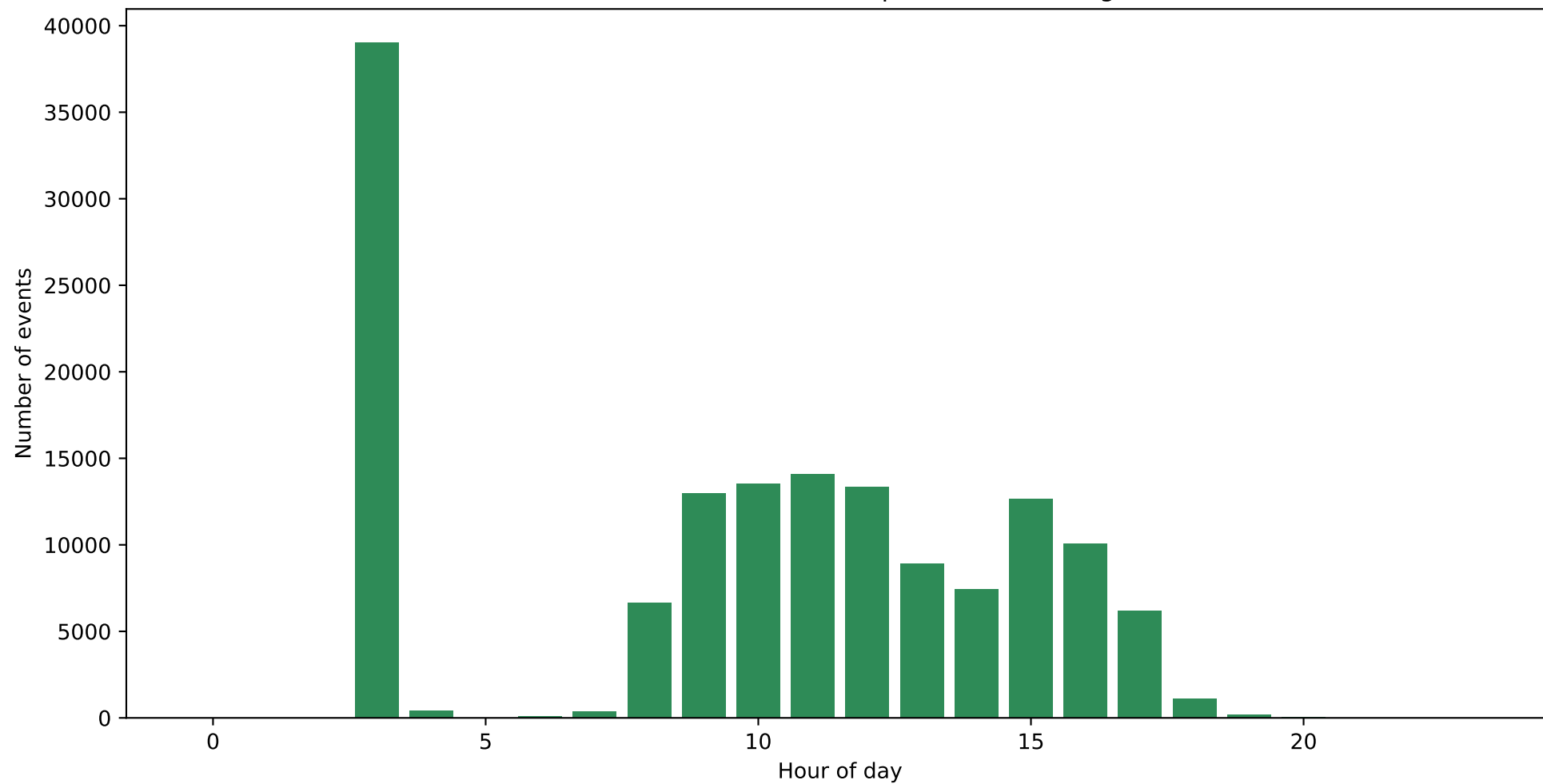
BAC - Role 3 (Authorization Requested) - Working hours
