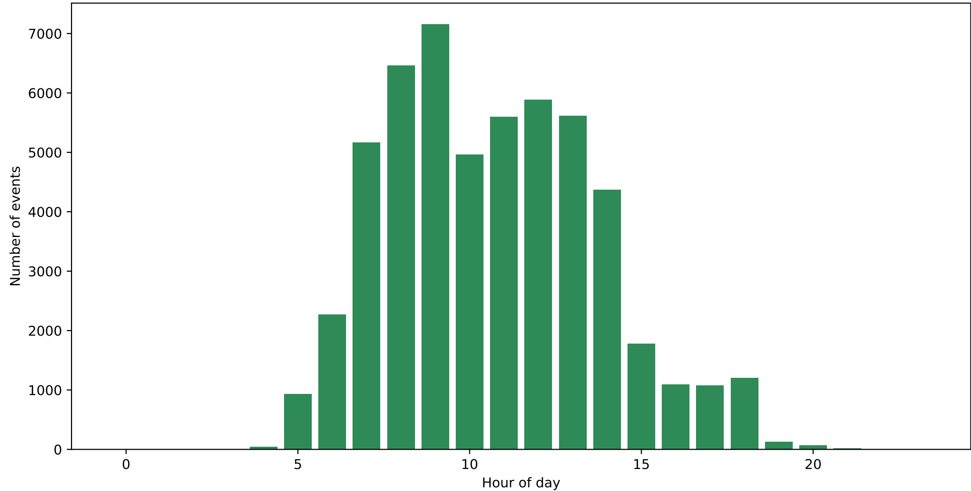
BPIC2017_After - Role 9 (A_Incomplete) - Working hours
