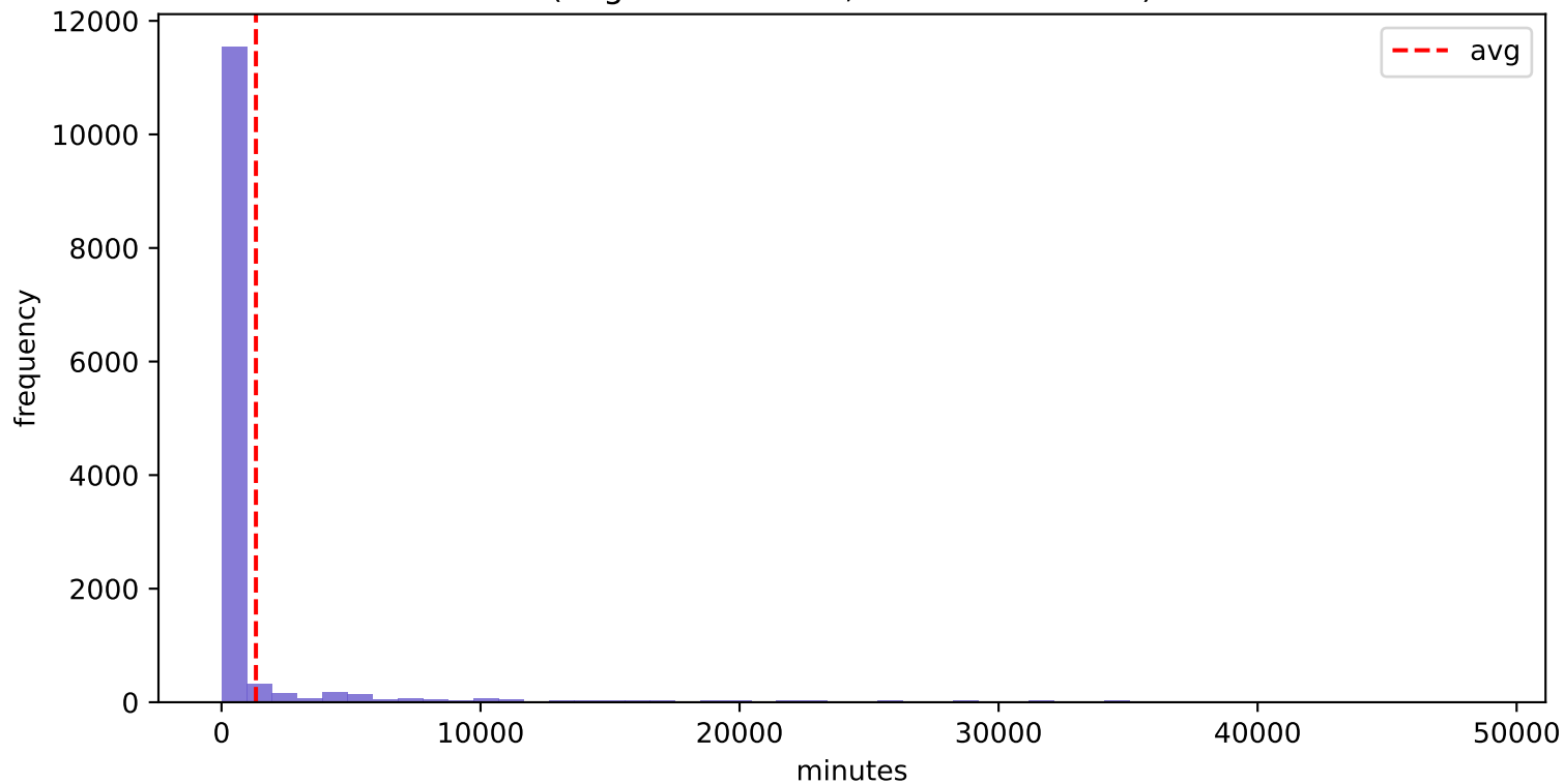
BPIC2017_Before - O_Create Offer (Avg 1328.85 min, Std 5083.28 min)
