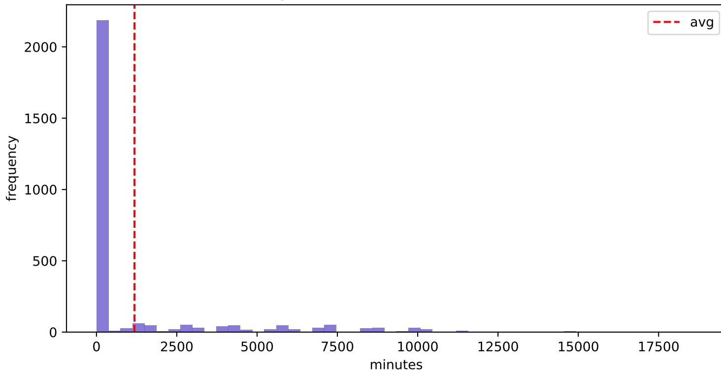
BPIC2017_After - W_Validate application (Avg 1183.67 min, Std 2653.50 min)
