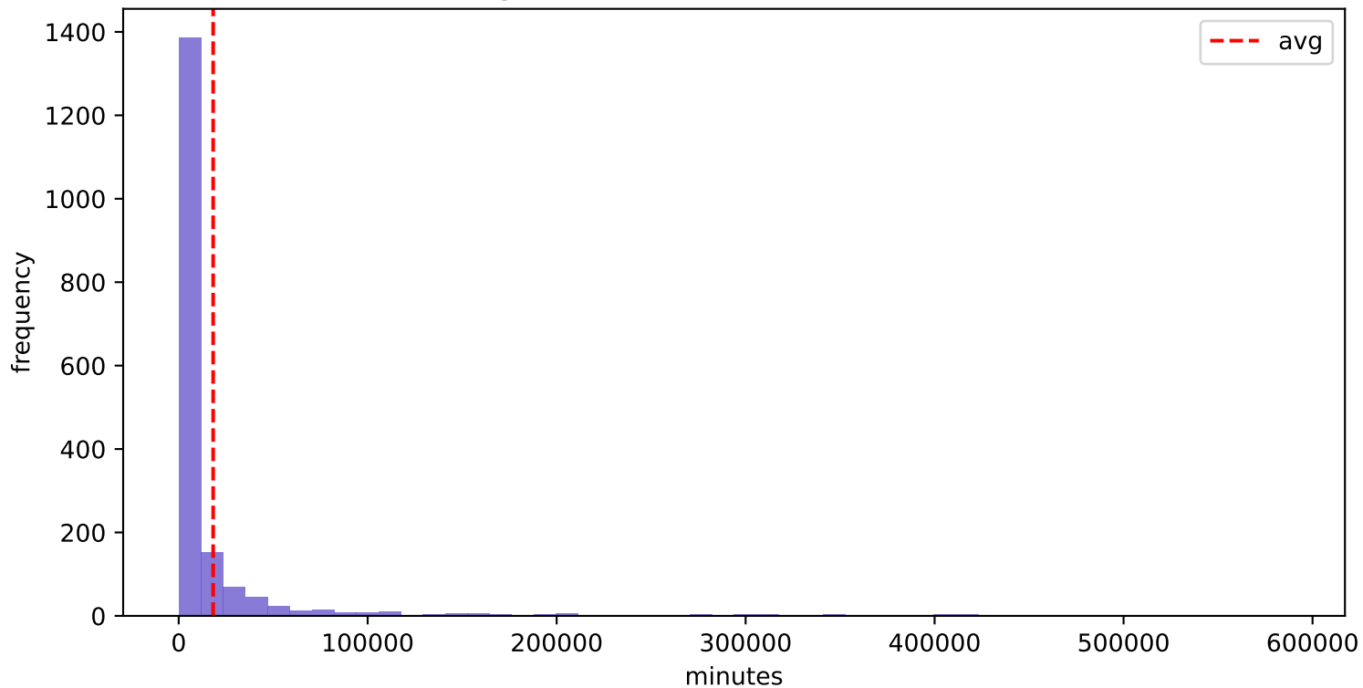
BAC - Network Adjustment Requested (Avg 18239.53 min, Std 57230.77 min)
