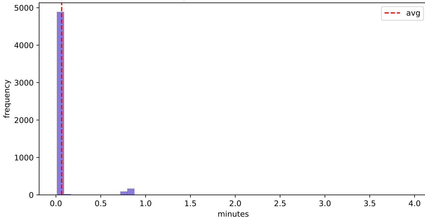
BPIC2012 - O_CREATED (Avg 0.06 min, Std 0.18 min)
