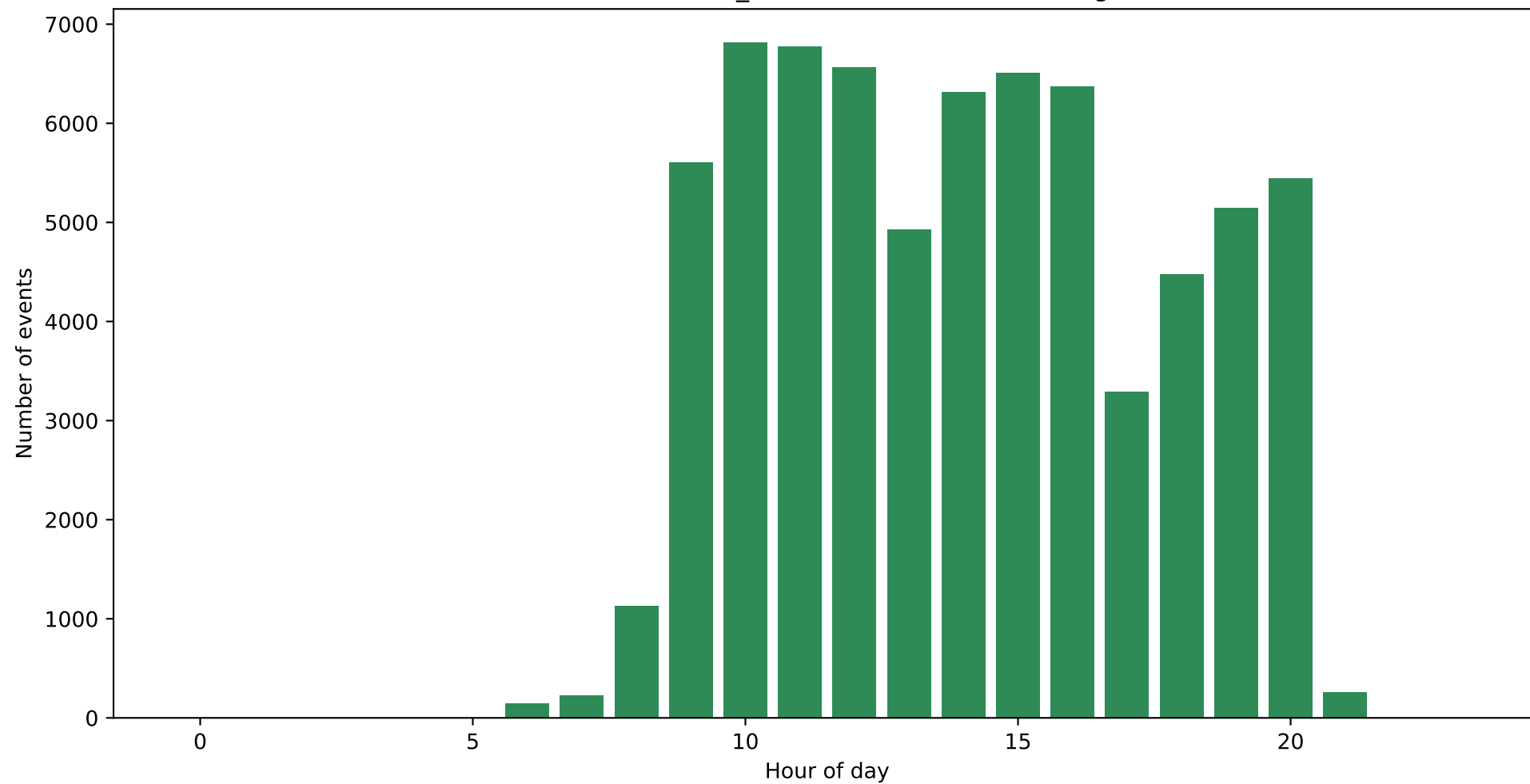
BPIC2012 - Role 9 (W_Afhandelen leads) - Working hours
