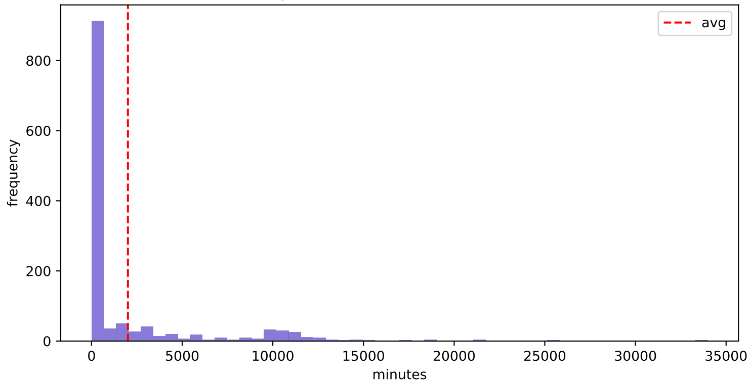
BPIC2012 - A_CANCELLED (Avg 2007.74 min, Std 4362.67 min)
