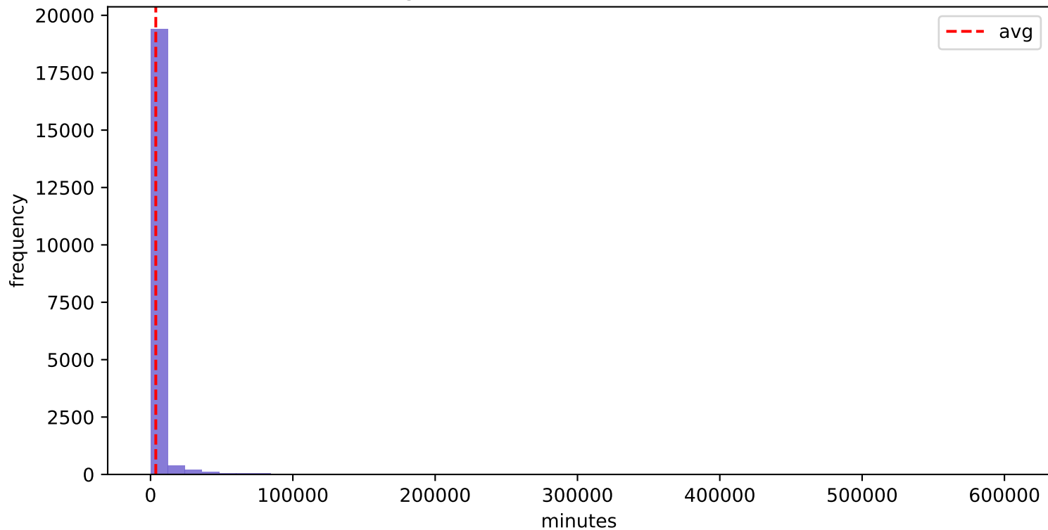
BAC - Service closure Request with network responsibility (Avg 3703.56 min, Std 24733.97 min)
