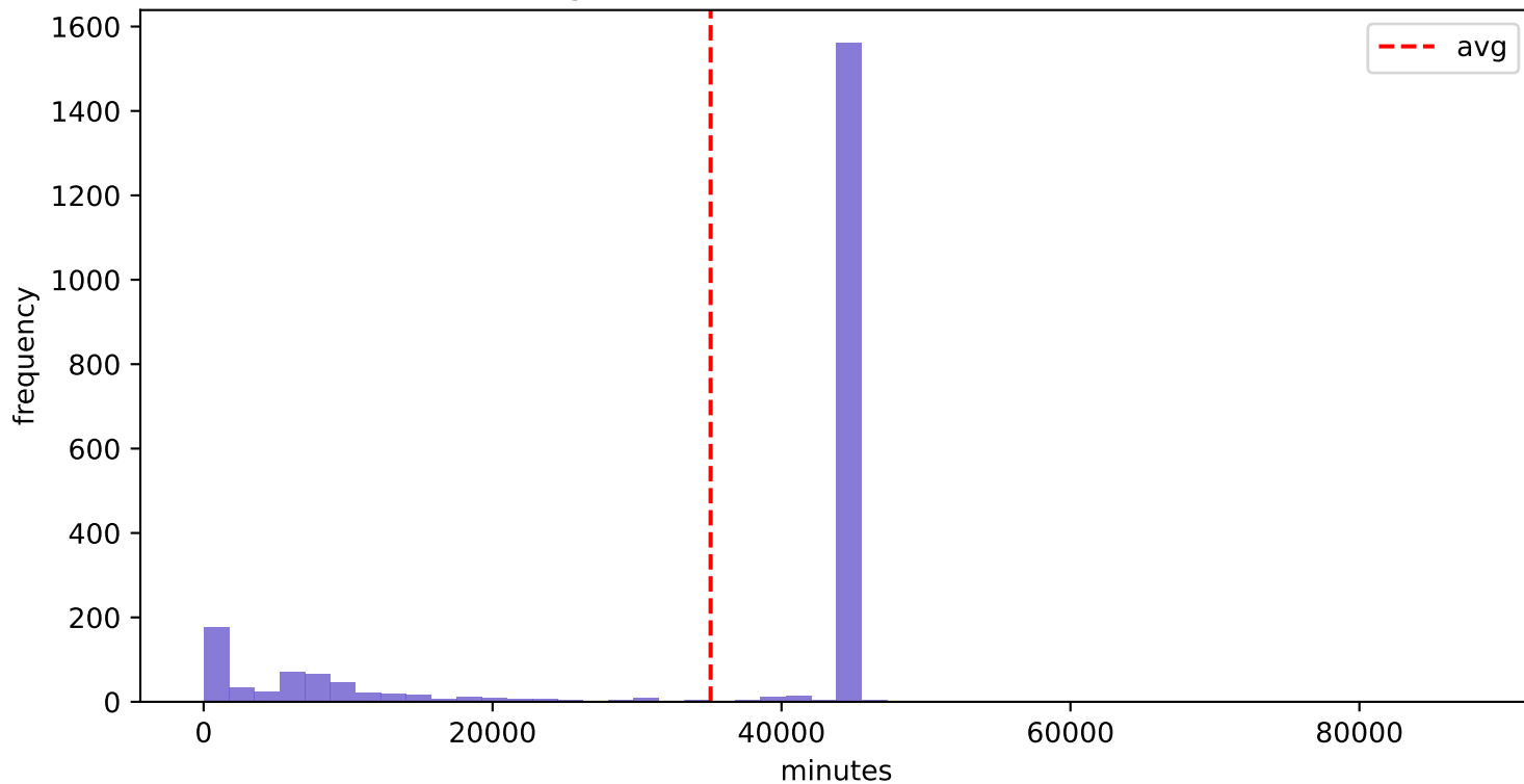
BPIC2017_After - A_Cancelled (Avg 35093.42 min, Std 16546.62 min)
