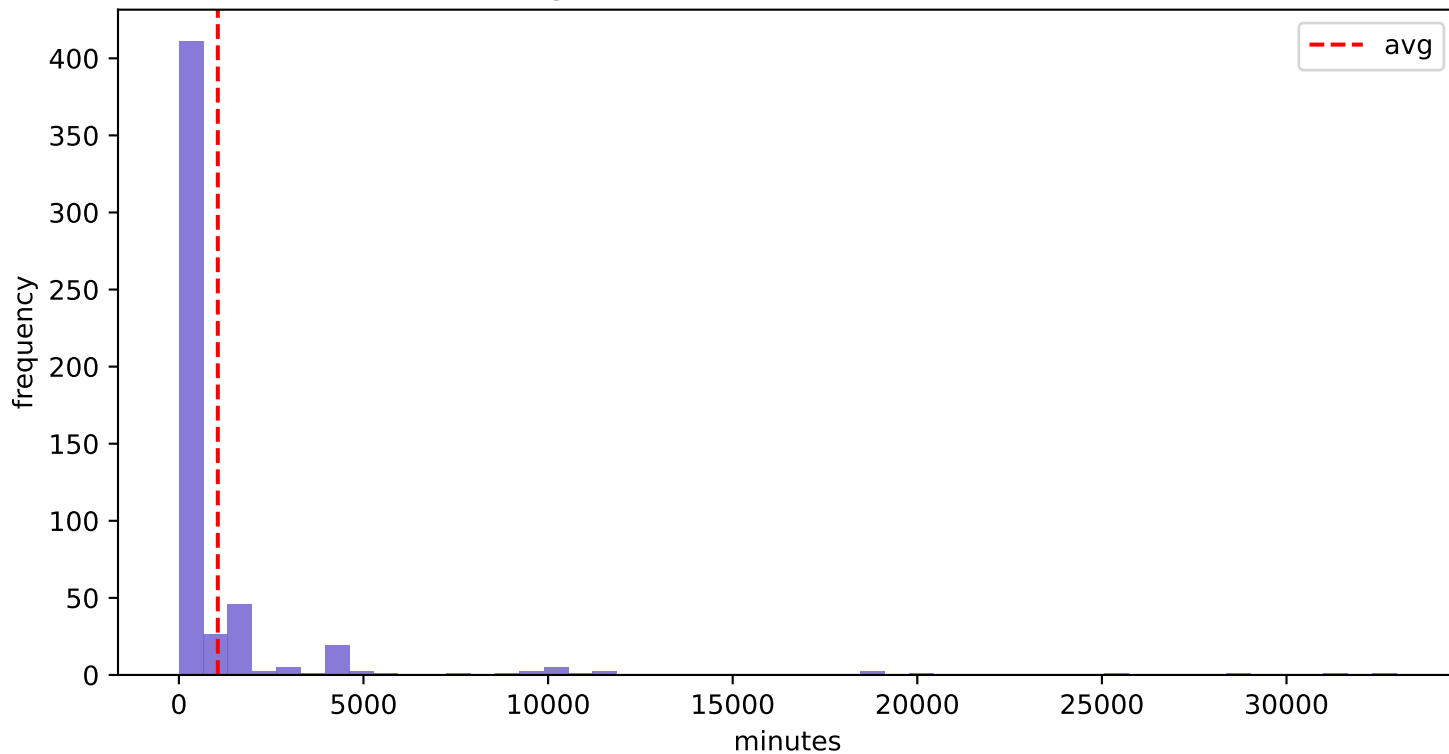
BPIC2017_After - W_Call incomplete files (Avg 1055.09 min, Std 3343.04 min)
