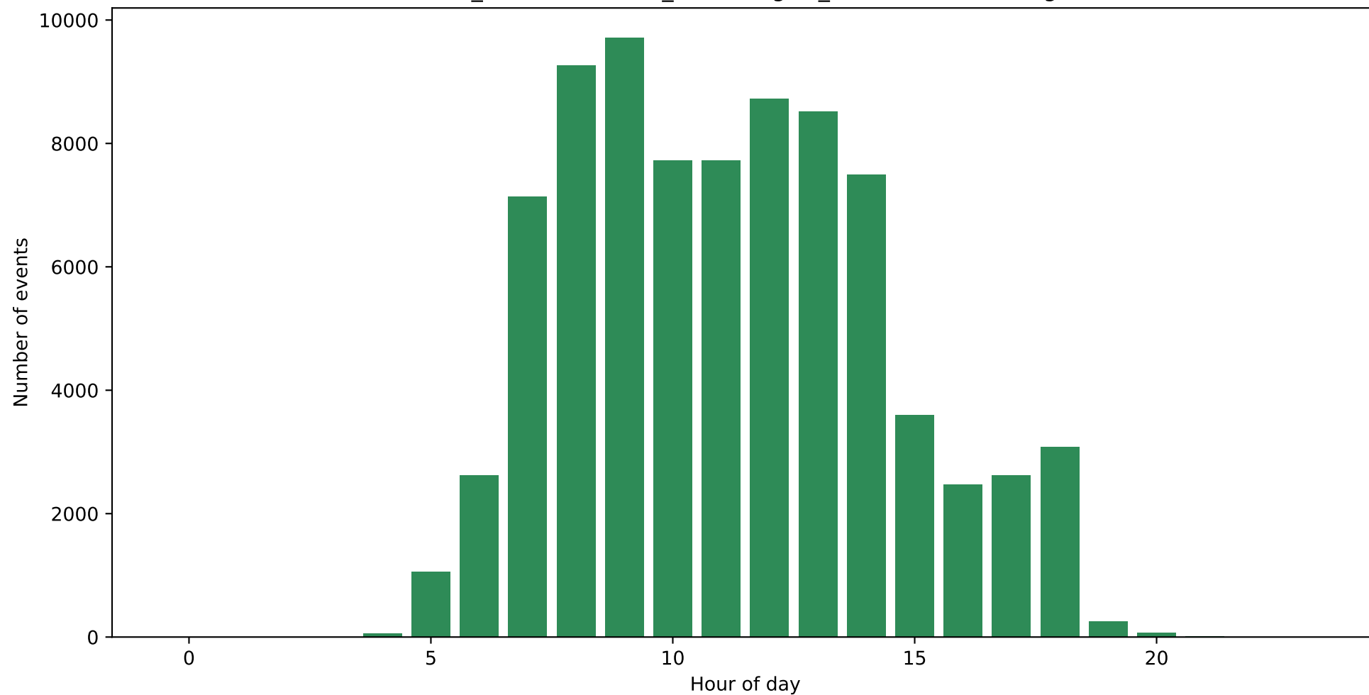
BPIC2017_After - Role 3 (A_Validating, O_Returned) - Working hours
