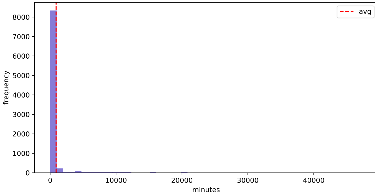
BPIC2017_After - O_Create Offer (Avg 893.54 min, Std 4172.50 min)
