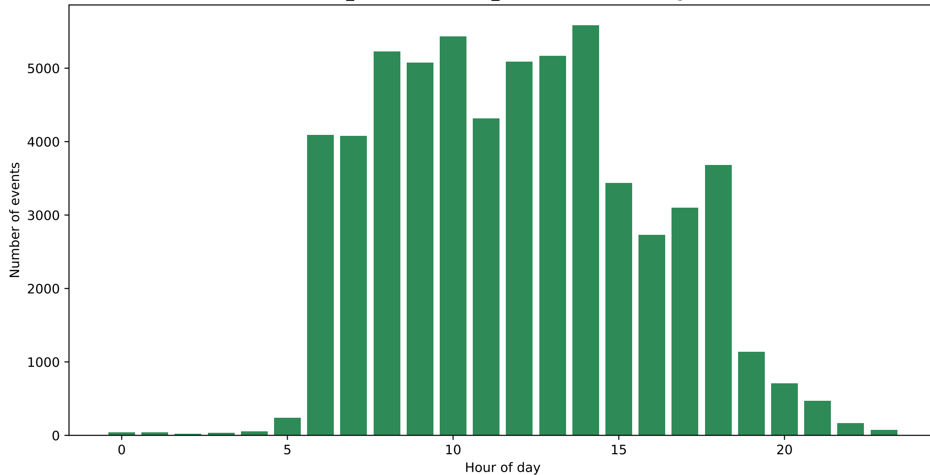
BPIC2017_After - Role 10 (W_Handle leads) - Working hours
