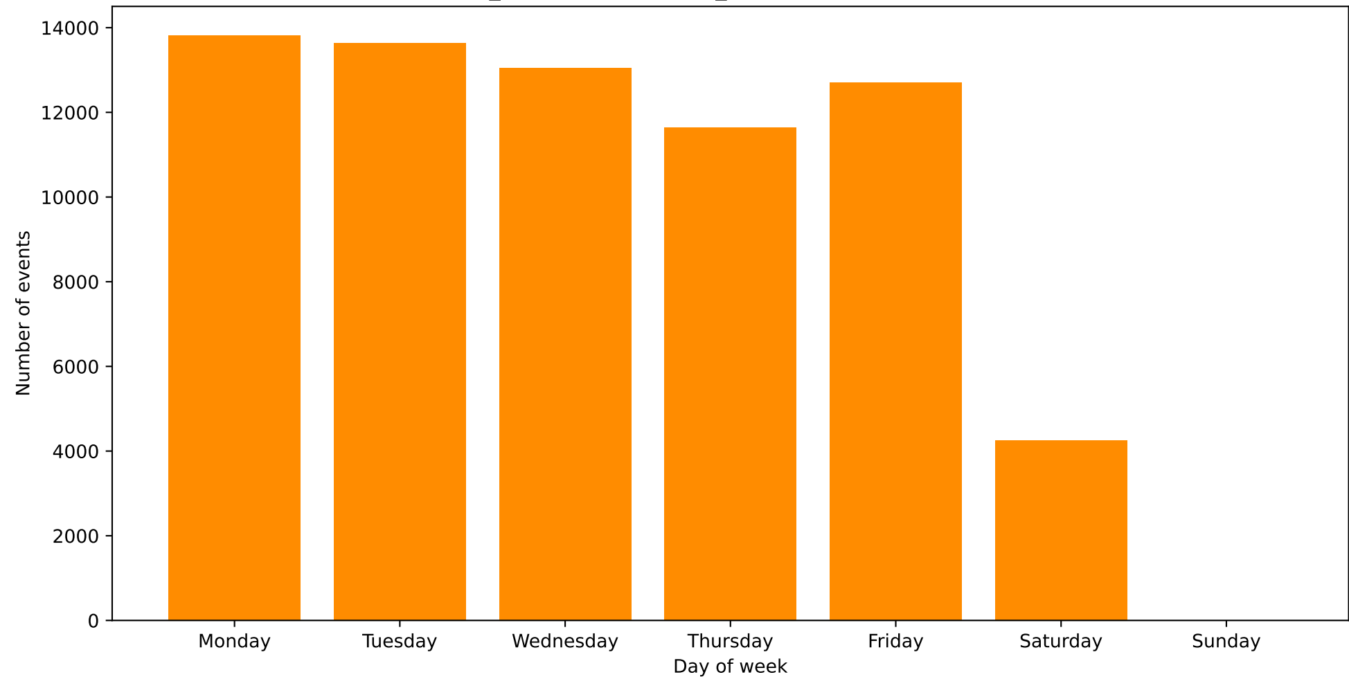
BPIC2017_Before - Role 11 (W_Call after offers) - Working days
