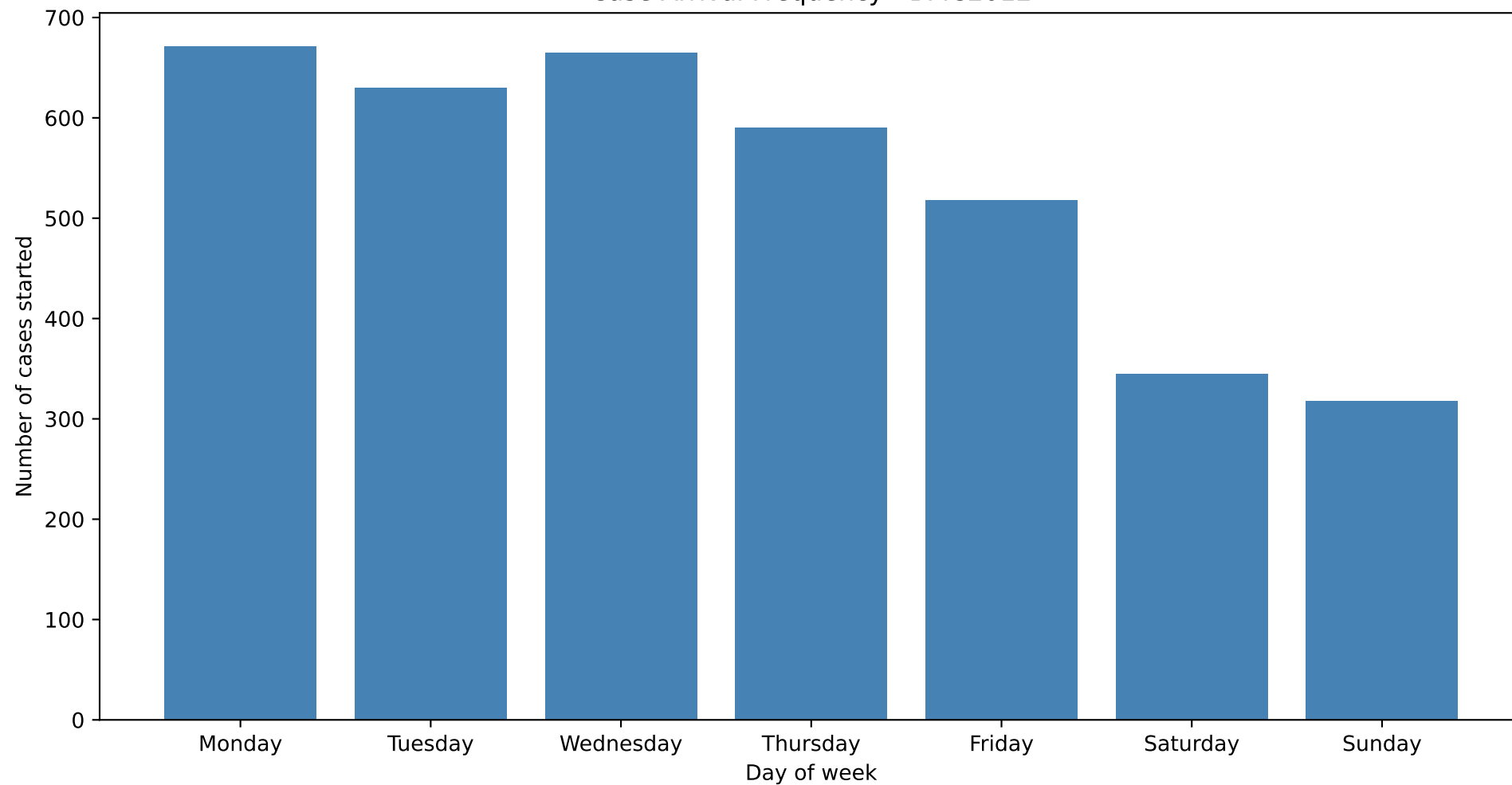
Case Arrival Frequency - BPIC2012
