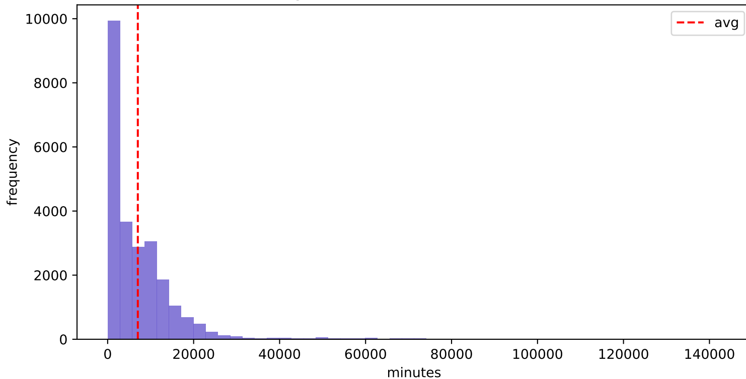
BAC - Service closure Request with BO responsibility (Avg 7017.29 min, Std 9331.64 min)
