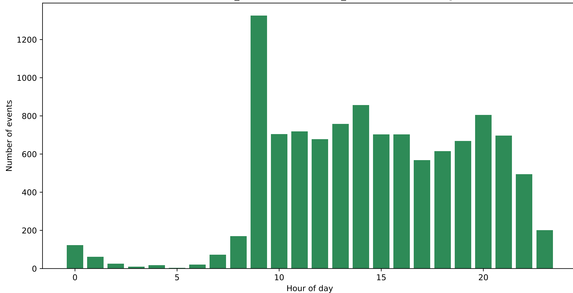
BPIC2012 - Role 4 (A_PARTLYSUBMITTED, A_SUBMITTED) - Working hours
