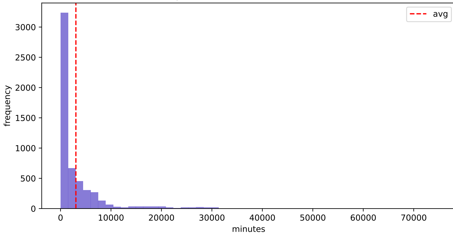
BPIC2017_Before - O_Accepted (Avg 3044.78 min, Std 5300.92 min)
