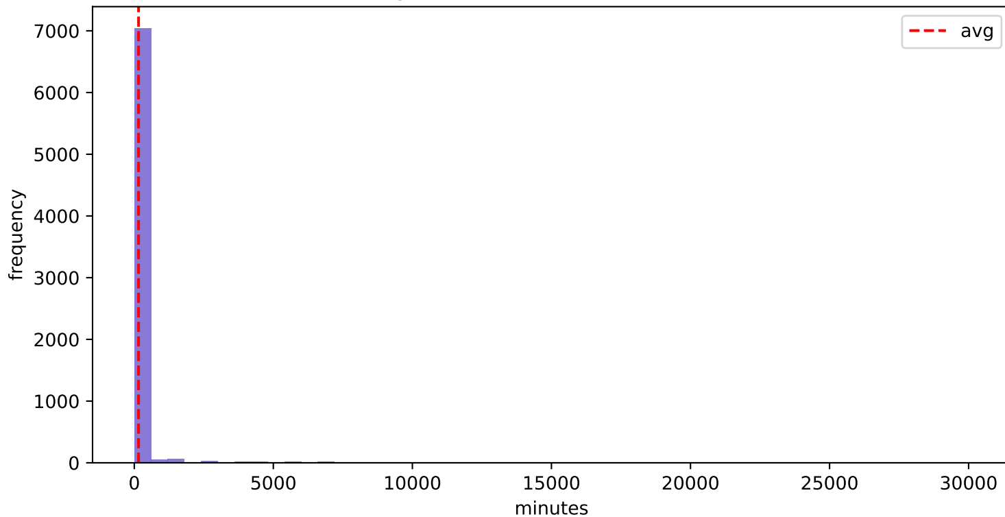
BPIC2017_Before - O_Returned (Avg 154.53 min, Std 1191.68 min)
