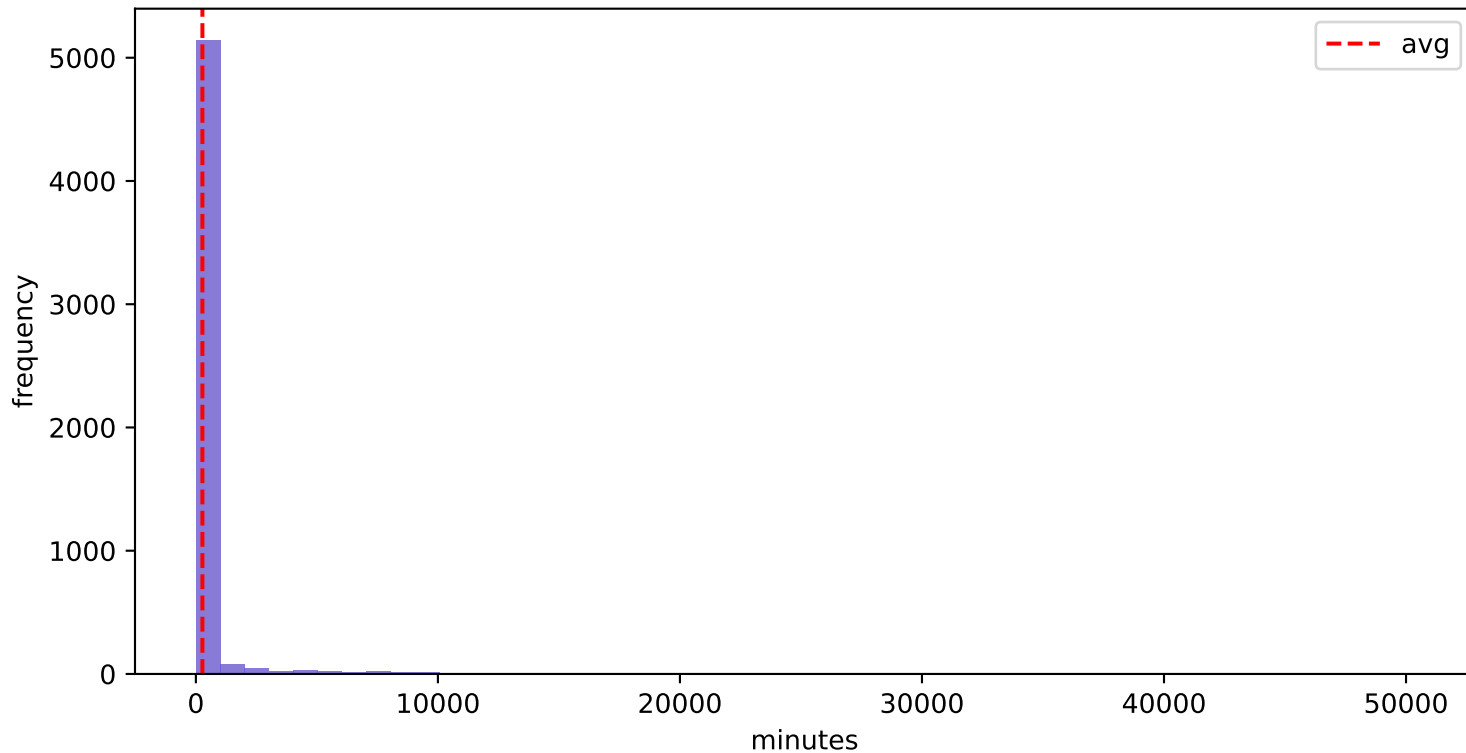
BPIC2017_After - O_Returned (Avg 270.16 min, Std 1684.35 min)
