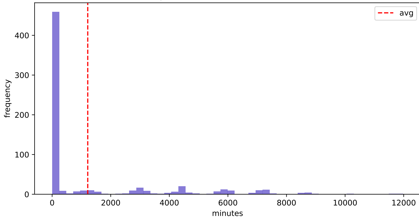
BPIC2012 - A_DECLINED (Avg 1215.77 min, Std 2321.14 min)
