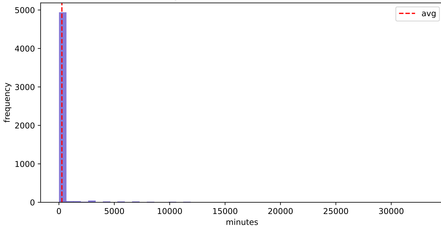
BPIC2012 - O_SELECTED (Avg 267.51 min, Std 1572.29 min)
