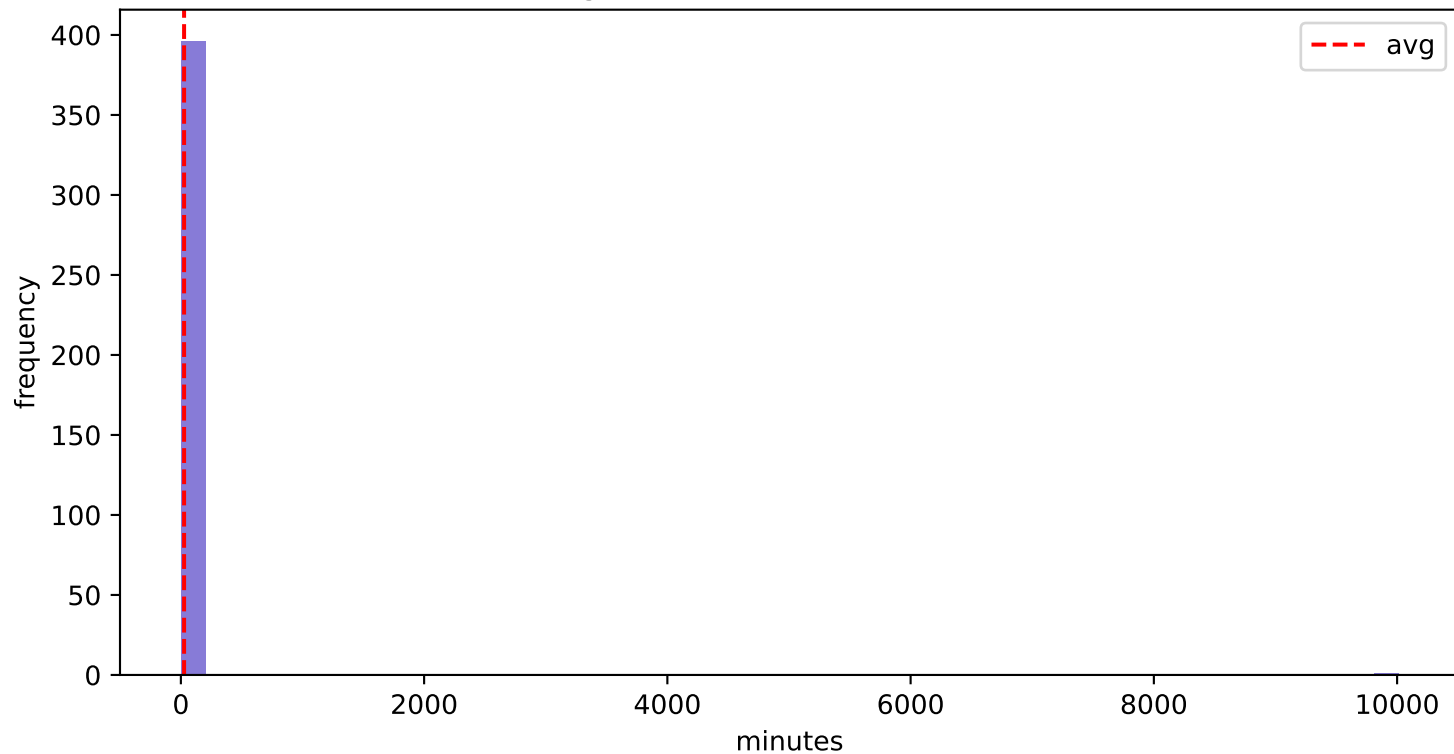
BPIC2017_After - O_Sent (online only) (Avg 26.45 min, Std 502.41 min)
