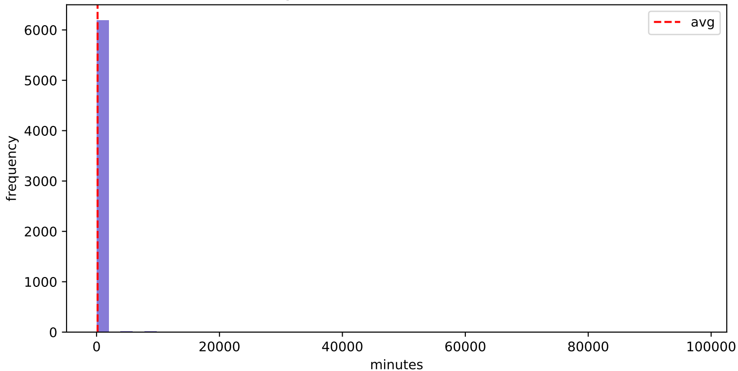
BPIC2017_Before - O_Cancelled (Avg 162.64 min, Std 2083.82 min)
