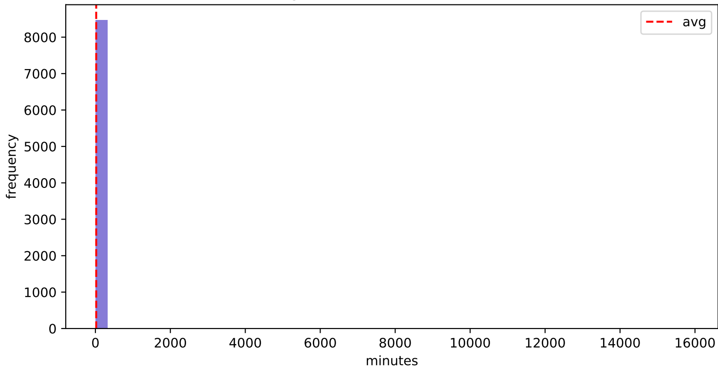
BPIC2017_After - O_Sent (mail and online) (Avg 20.98 min, Std 351.92 min)
