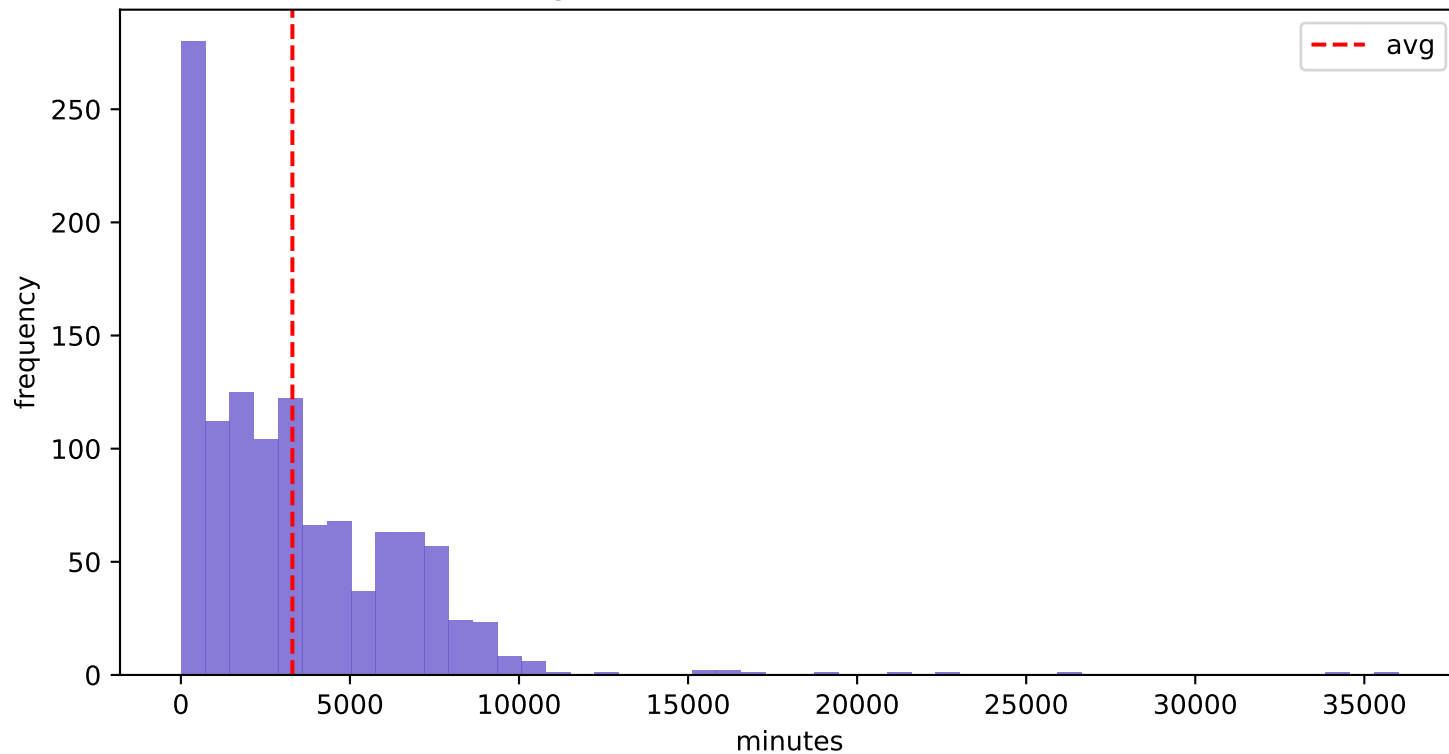
BPIC2017_Before - A_Denied (Avg 3298.62 min, Std 3295.37 min)
