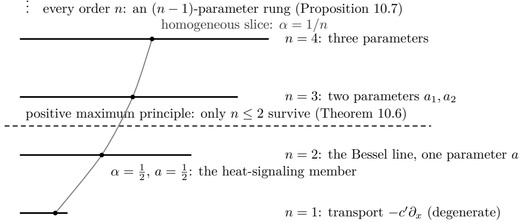
Figure 8: The ladder of local media. Locality alone admits media of every order: rung n is the (n - 1) -parameter family of Proposition 10.7, with n = 1 the degenerate transport member. The positive maximum principle cuts the ladder between orders two and three (Theorem 10.6), leaving the transport member and the Bessel line. The homogeneous (semigroup) members are one point per rung, the stable cases \alpha = 1/n of [8] (Remark 10.9); the maximum principle acts on them the same way, and what survives of the slice is the single point \alpha = \frac{1}{2} — the heat-signaling equation — which under the hemigroup axioms unfolds into the full Bessel rung.
