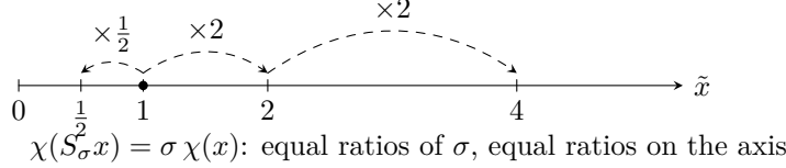
Figure 4: The orbit coordinate. (a) On the scale axis as the family presents it, the action S_\sigma of (A8) is some increasing bijection; the orbit of the point 1, \sigma \mapsto S_\sigma 1 , is continuous, strictly increasing and has no fixed point, so it sweeps the whole axis (Lemma 6.2, Proposition 6.3). Equal ratios of \sigma are unequal steps on the axis. (b) Labelling each point by the \sigma that reaches it, \tilde{x} = \chi(x) , the same action becomes multiplication by \sigma : the canonical gauge. In this gauge every accumulated exponent is a dilate of one function, G(x, s) = F(\tilde{x}s) .
