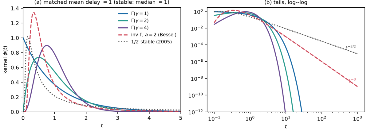
Figure 10: Time-causal scale-space kernels at matched mean delay 1 (stable: median 1, its mean being infinite). (a) linear scale; (b) log-log, with the power-law guides t^{-3} (inverse-gamma, a = 2 ) and t^{-3/2} ( \frac{1}{2} -stable).
