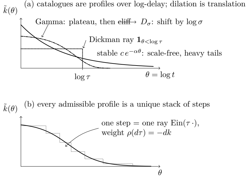
Figure 3: Delay catalogues in the log-delay coordinate \theta = \log t , where the Lévy measure k(t) t^{-1} dt becomes the profile \tilde{k}(\theta) = k(e^\theta) and dilation acts by translation. (a) Full scale covariance requires only that the profile be nonincreasing — zooming out may only add delay intensity (Lemma 7.1); within that freedom the named families are shapes: the stable family is the exactly scale-free exponential profile, whose slow decay is the heavy tail (Corollary 7.4); the Gamma family cuts long delays off at a cliff, buying finite moments; and the Dickman ray is a log-uniform band of delays with a hard cutoff. (b) The Dickman superposition (Lemma 7.7): every nonincreasing profile is a unique positive stack of unit steps, so every admissible family is a unique superposition of drift and dilated Dickman subordinators, with mixing measure \rho = -dk (Proposition 7.8).
