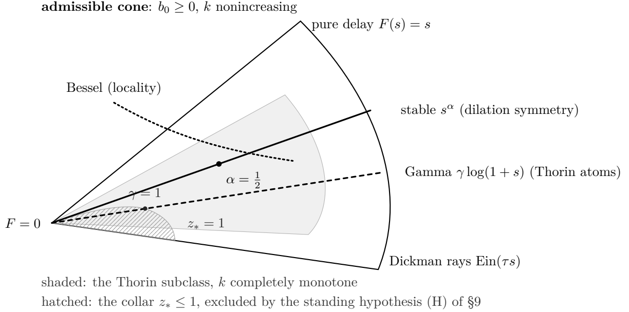
Figure 5: The admissible cone. Theorem 7.3 identifies the exponents F with pairs (b_0, k) , a drift and a nonincreasing density; these form a convex cone (Lemma 7.6) whose extreme rays are the Dickman rays \text{Ein}(\tau \cdot) and the pure delay (Proposition 7.8). Inside it, the exponents with completely monotone k form the Thorin subclass. None of the three distinguished families of the paper is extreme; each is a slice cut by a different principle — the stable exponents s^\alpha by dilation symmetry (Corollary 7.4), the Gamma family as the atoms of the Thorin representation, the Bessel family by locality (§10) — and the stable and Bessel slices meet at \alpha = \frac{1}{2} , the heat-signaling member, which is the one point the semigroup axioms allowed on the memory line. The hatched collar at the apex is excluded by the standing hypothesis (H) of §9 (Definition 9.1). Unlike the Thorin condition, which selects rays and so cuts a subcone, (H) cuts across rays: z_* is homogeneous of degree one along them (Lemma 9.4), so a ray of finite z_* enters (H) beyond the threshold multiple 1/z_* , and the excluded set \{z_* \leq 1\} is a collar around the apex — pinching to nothing on every exponent with drift and on the stable and Bessel slices, where z_* = \infty , reaching the unit point of each Dickman ray, where z_* = k(0^+) = 1 , and crossing the Gamma ray at \gamma = 1 . The drawing is schematic: the cone is infinite-dimensional.
