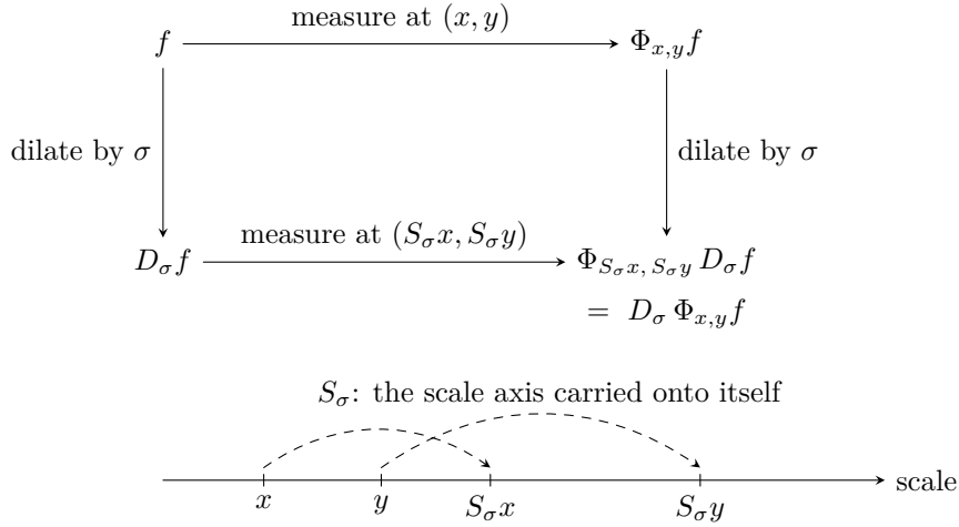
Figure 1: Scale covariance (A8). Dilating the signal by \sigma and then measuring is the same as measuring and then dilating, provided the measurement is taken at the transported scales (S_\sigma x, S_\sigma y) : the square commutes. The lower strip shows the relabelling. Nothing ties the scale labels to a unit of time at this stage, so (A8) can only ask that the family be mapped onto itself, with the labels rearranged by some increasing bijection S_\sigma ; §6 shows that the axioms determine S_\sigma and thereby a canonical parametrization of the scale axis.
