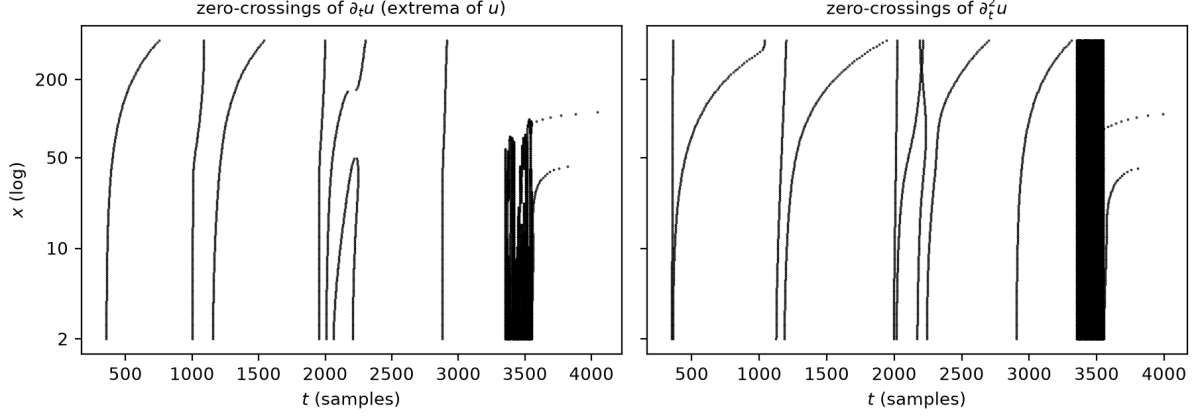
Figure 14: The fingerprints of the same run: zero-crossings of \partial_t u (the extrema of u , left) and of \partial_t^2 u (right) across scale. The classical picture — arches closing from below, never re-opening — holds in this run, sheared rightward along the delay direction: the causal counterpart of the Gaussian fingerprint diagrams. The noise burst’s dense column annihilates pair by pair; the wake companion’s arch closes at x \approx 50 .
