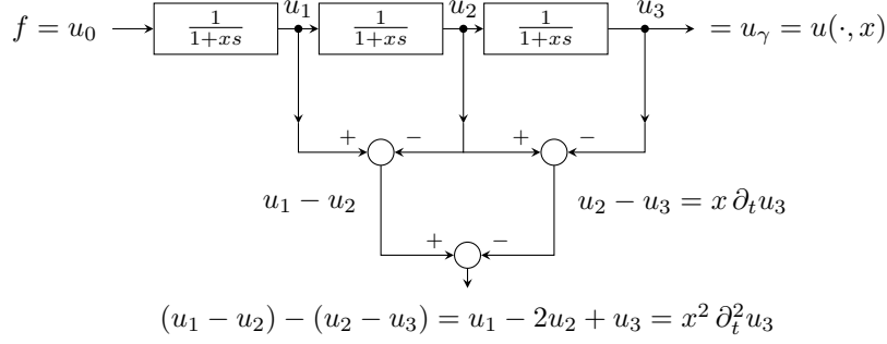
Figure 12: Jets by subtraction along the shape column ( \gamma = 3 ). The column of \gamma identical leaky integrators at time constant x — the pure-pole cascade from scale zero, the gamma memory of [39] — carries the fields u_0, \dots, u_\gamma of increasing shape as coexisting states. The scale-normalized jet at scale x is read off the taps by binomial-weighted subtraction, x^n \partial_t^n u_\gamma = \sum_j (-1)^{n-j} \binom{n}{j} u_{\gamma-j} , realized as iterated differences of adjacent taps (Proposition 12.4): no temporal differencing, and no second memory, anywhere in the architecture.
