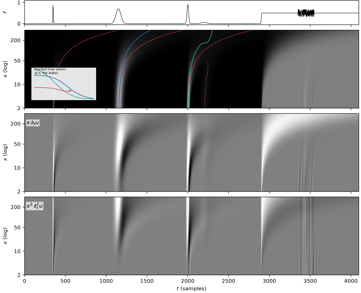
Figure 13: The machine run end to end (Example 12.7): the Gamma cascade at \gamma = 2 on a synthetic gray-level signal, in the orientation of Figure 7 — time horizontal, \log x vertical, the signal entering along the bottom edge. Top: the input. Second panel: the field u , with the mean-delay curves t_0 + \gamma x of the three isolated events (dashed), the tracked maxima of the strong (teal) and coarse (blue) events, and the wake companion's track (red, dotted); the inset plots the tracked values against scale — nonincreasing while past-dominating, the wake curve (magnified 6\times ) showing the echo uptick before its annihilation ( \times ). The bend near the top of the strong event's track is its arch merging with a neighbour — structure, not a tracking failure. Lower panels: the scale-normalized jet maps x \partial_t u and x^2 \partial_t^2 u , computed by binomial subtraction along the shape column (Proposition 12.4); for the fine streaks under the noise burst in the second-order map, see the example's closing paragraph.
