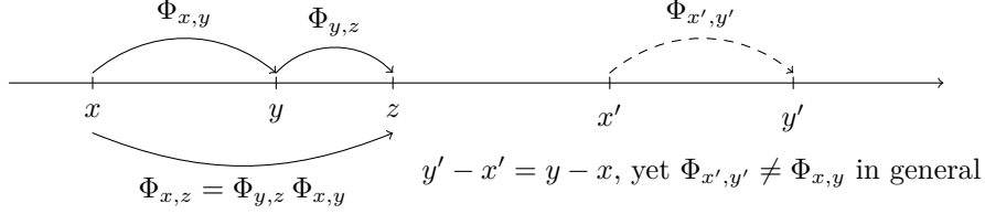
Figure 2: The two readings of the cascade property. (a) In the semigroup form the increment is indexed by an amount of scale: composition adds amounts, and increments of equal amount are the same operator wherever they act — the axis positions carry no labels because the operators cannot see them. (b) In the hemigroup form the increment is indexed by an interval of the scale axis: composition joins adjacent intervals, and increments of equal span at different positions need not coincide. The axioms retain what the two forms share — a measurement of a measurement is a measurement — and drop the rest.
