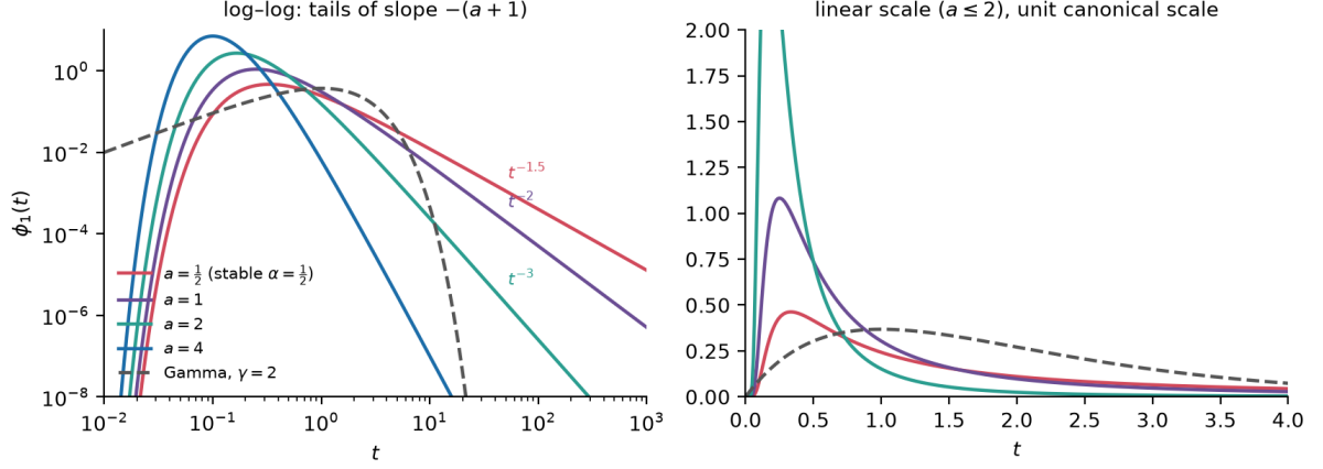
Figure 6: The moment threshold, seen in the tails. Left, log-log: the kernels \phi_1 of the Bessel family of Proposition 8.17 for shapes a = \frac{1}{2}, 1, 2, 4 are straight lines of slope -(a+1) at large t , so the moments of order n < a are finite and no others; a = \frac{1}{2} is the extremal stable member of the semigroup theory, the heaviest tail in the family, with no mean. The dashed curve is the Gamma kernel with \gamma = 2 : an exponential tail, every moment finite (Proposition 8.12). Right: the same kernels on a linear scale at unit canonical scale. Raising a buys moments at the price of temporal reach — a heavier tail is a longer scale-invariant memory, not a defect. The comparison at matched delay, which is what an implementation sees, is in §11.
