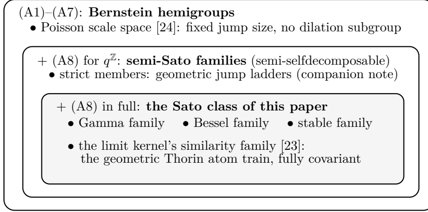
Figure 15: The three-level stratification of Remark 13.1. The axioms without covariance admit the Bernstein hemigroups, where the Poisson scale space lives and stays; covariance under a discrete subgroup q^{\mathbb{Z}} cuts out the semi-Sato stratum, whose strict members are geometric refinements of it; full continuous covariance cuts out the class characterized in this paper, which contains the similarity family generated by the time-causal limit kernel's exponent. Containment, not competition: the earlier constructions occupy strata of one axiom system.
