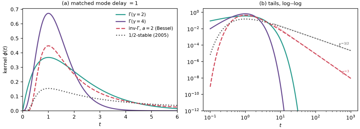
Figure 11: The same comparison at matched mode delay = 1, the normalization of the 2005 influence-curve discussion. (a) linear scale; (b) log-log, with the exact power-law asymptotes.
