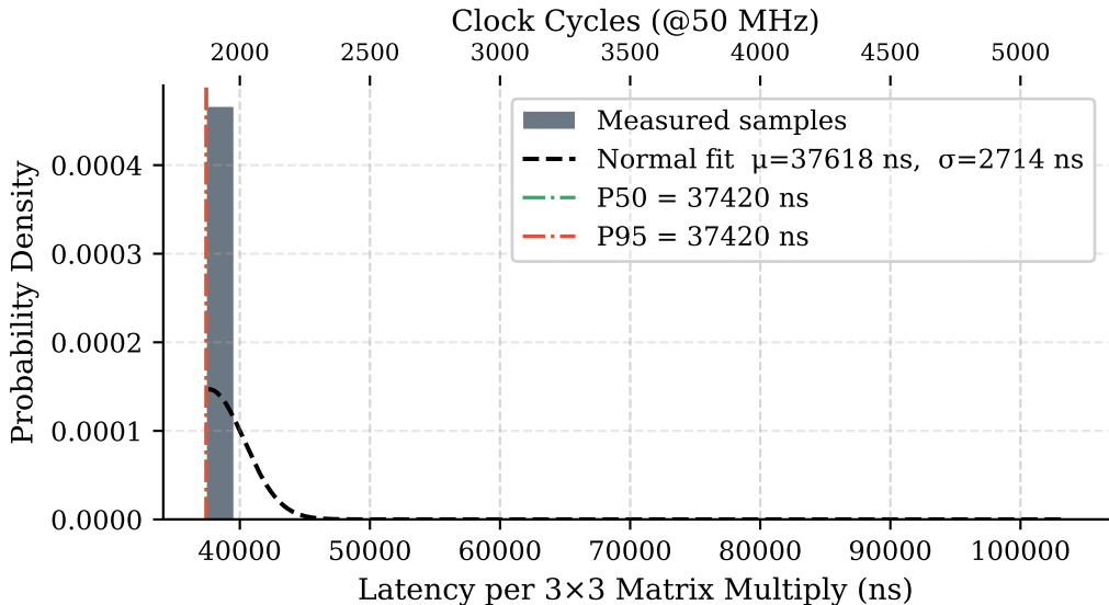
Fig. 1 – 3×3 Array Latency Distribution (1 000 matrix multiplies, flush each, LW-HPS2FPGA bridge)
