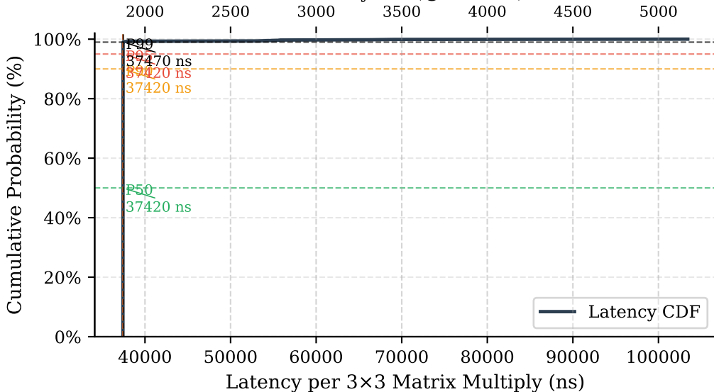
Fig. 2 - Latency CDF (3×3 Array, 1 000 samples) Clock Cycles (@50 MHz)
