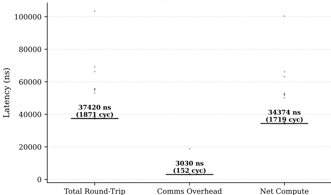
Fig. 3 – Latency Breakdown: Total vs. Comms vs. Net Compute (3×3 Array, 1 000 samples each)
