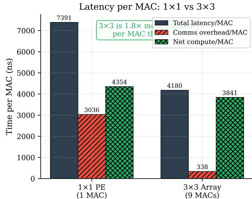
Fig. 6 - 1\times 1 PE vs 3\times 3 Array: Efficiency Comparison
