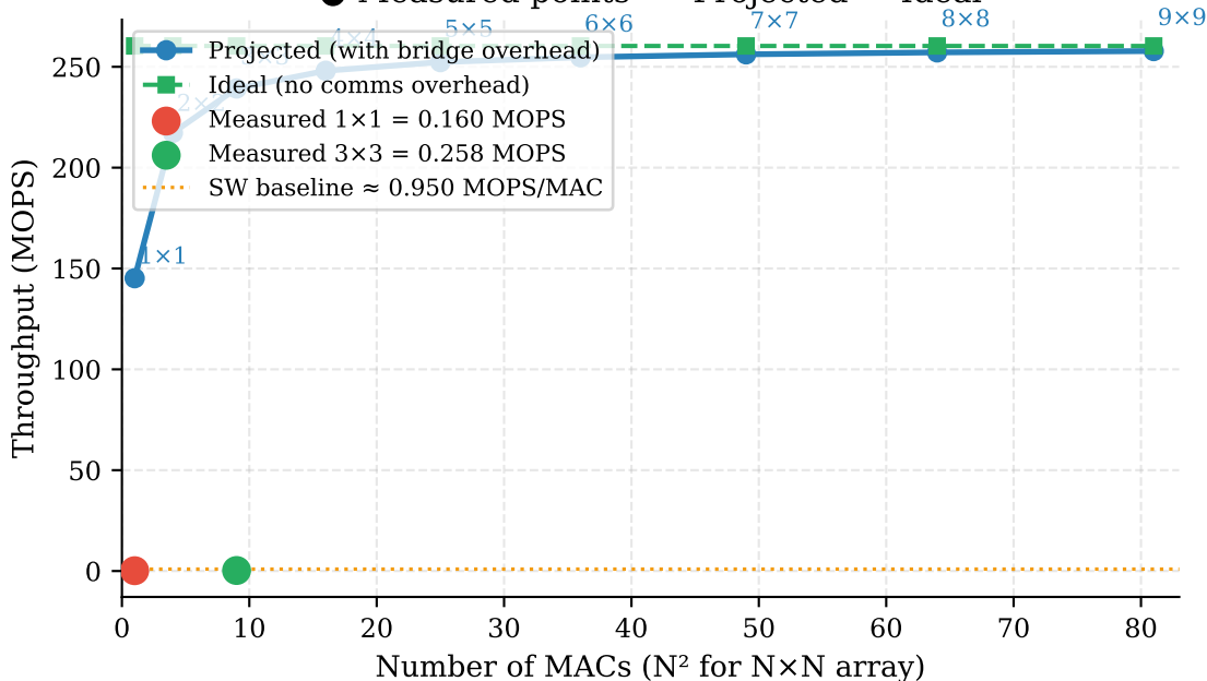
Fig. 7 – Throughput Scaling Projection (fixed bridge overhead amortised over N^2 MACs)
