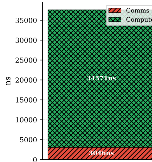
Time Breakdown
