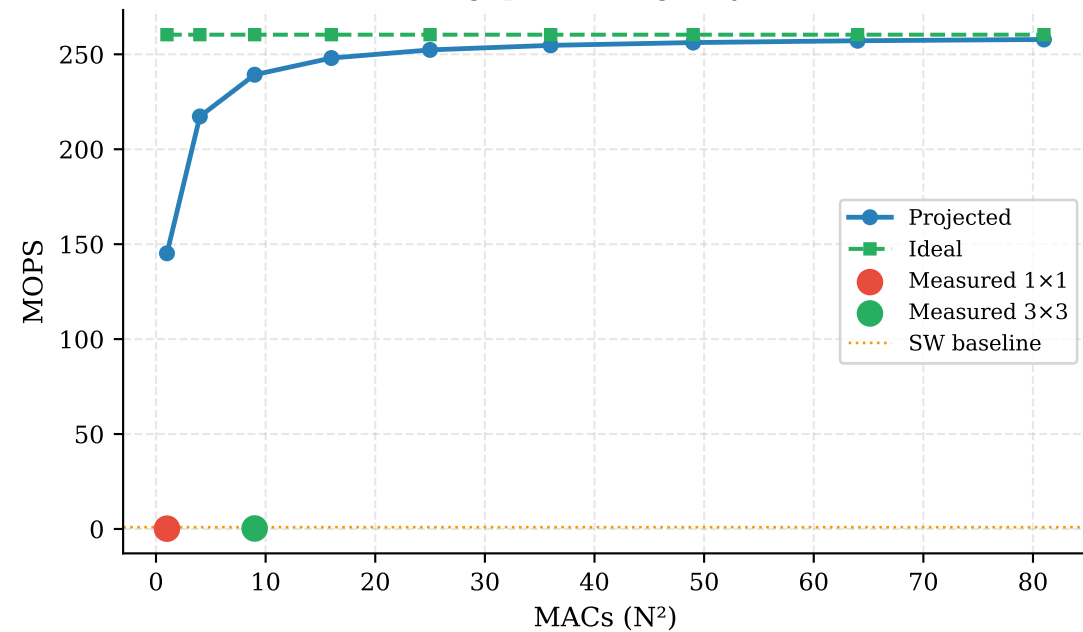
Throughput Scaling Projection
