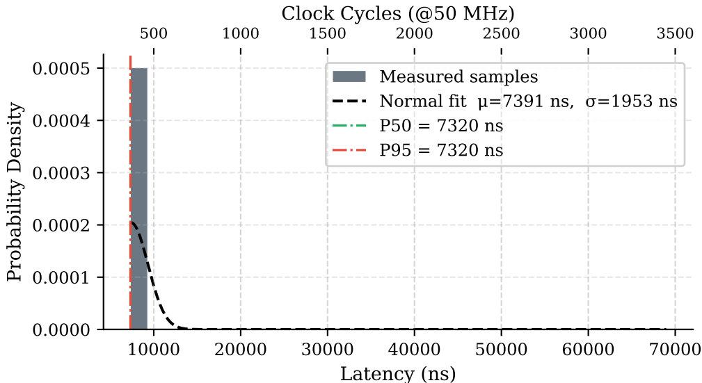
Fig. 1 - IP_PE Operation Latency Distribution (1×1 PE, LW-HPS2FPGA bridge, Linux userspace)
