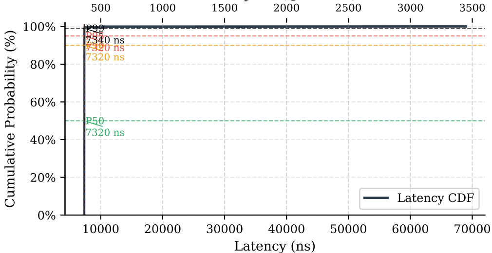
Fig. 2 - Latency CDF (1×1 PE, 1 000 samples) Clock Cycles (@50 MHz)
