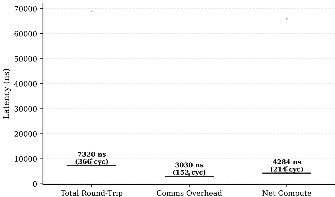
Fig. 3 – Latency Breakdown: Total vs. Communication vs. Compute (1×1 PE, 1 000 samples each)
