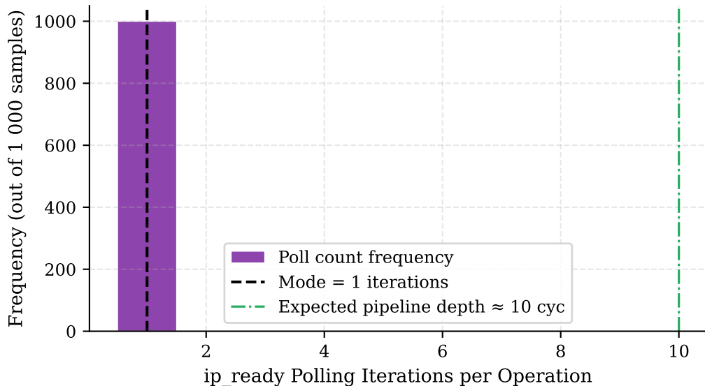
Fig. 5 – ip_ready Polling Distribution (validates FSM pipeline determinism)
