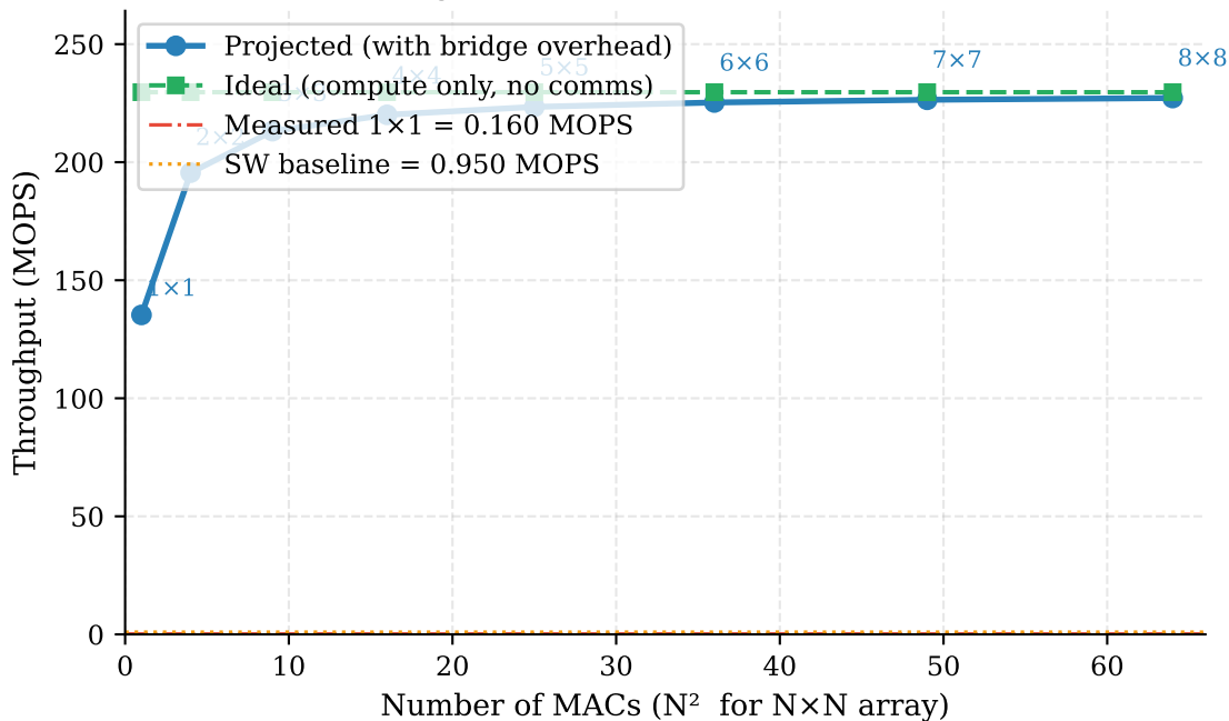
Fig. 6 – Throughput Scaling Projection (fixed bridge overhead amortised over N^2 MACs)
