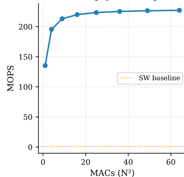
Throughput Scaling
