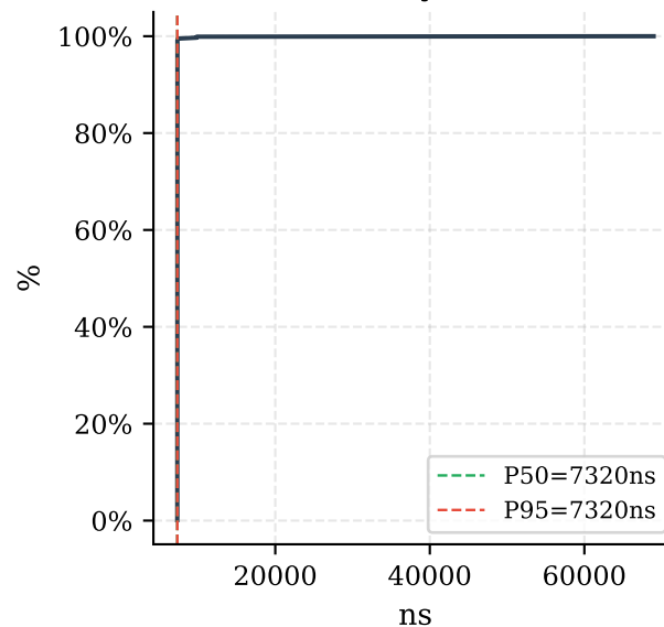
Latency CDF
