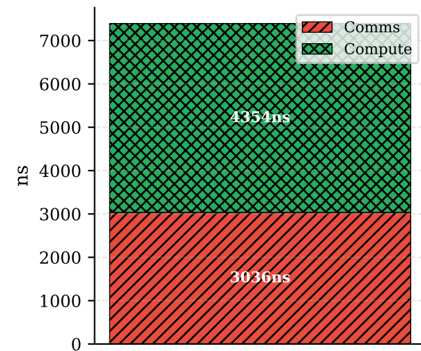
Time Breakdown
