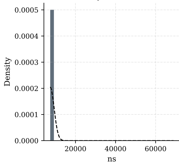
Latency Distribution
