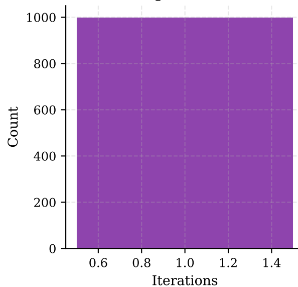
Polling Distribution
