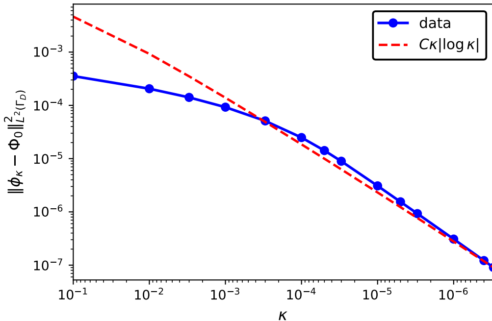
L^2 boundary convergence
