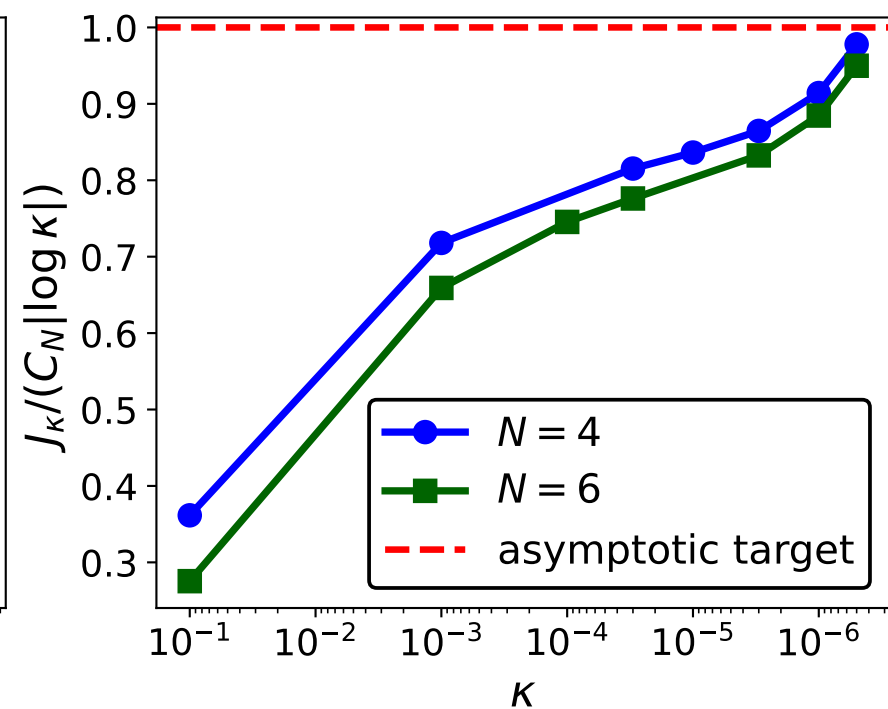
Exact-constant ratio
