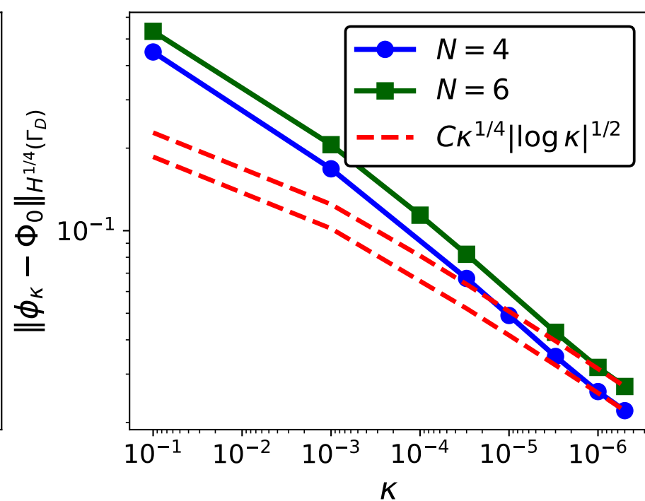
H^{1/4} boundary convergence
