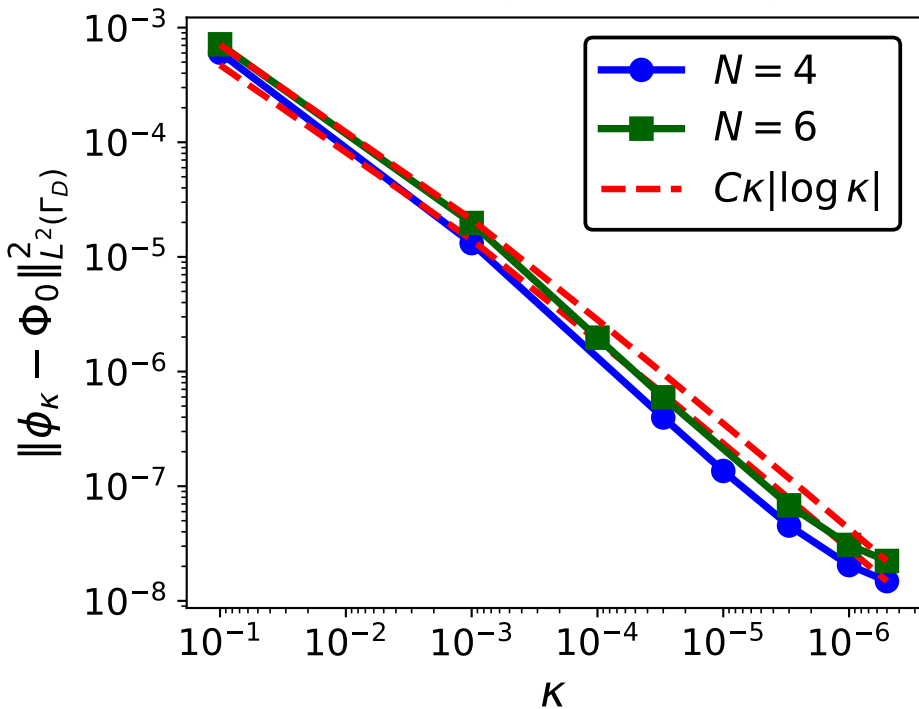
L^2 boundary convergence
