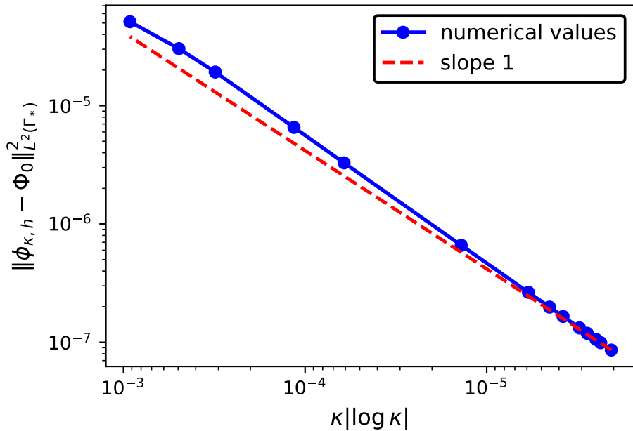
L^2 boundary convergence
